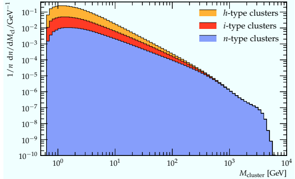
(b) Contributions of the cluster classes to the invariant cluster mass distribution in soft-inclusive pp collisions at 7 TeV.
