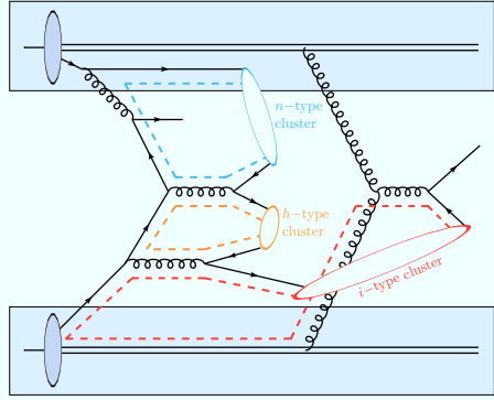
(a) Sketch of cluster classes in a simple pp event. The classes are defined in the text.
