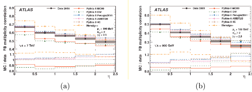
Figure 1: Forward-backward multiplicity correlation in symmetrically opposite \eta intervals for events with at least two charged particles with p_T > 100 MeV and |\eta| < 2.5 . Data at 7 TeV (a) and 900 GeV (b), compared to a selection of MC simulations [5].
