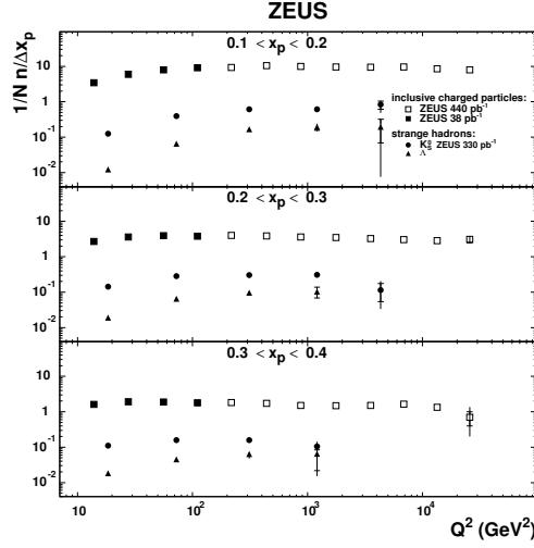
Figure 4: The measured scaled momentum distributions (1/N)(n(H)/\Delta x_p) for H = K_S^0 (dots), \Lambda (triangles) and light charged particles (squares) as functions of Q^2 in different regions of x_p . Other details as in the caption to Fig. 2.
