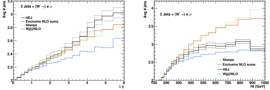
Figure 2: A comparison of the predictions for the average number of jets in an inclusive W +di-jet sample from different theoretical descriptions as a function of (left) the difference in rapidity between most forward and most backward jet, and (right) as a function of H_T . Plots taken from [12].
