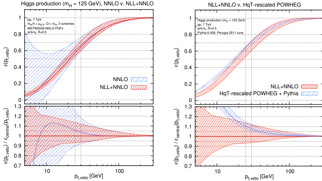
Figure 1: Left: the jet-veto efficiency for Higgs production at order \alpha_s^2 (NNLO) and matched to NLL resummation (NLL+NNLO). Right: NLL+NNLO efficiency compared to POWHEG rescaled using HqT.
