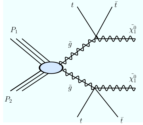
Figure 1: Model A1 with three body decays.
