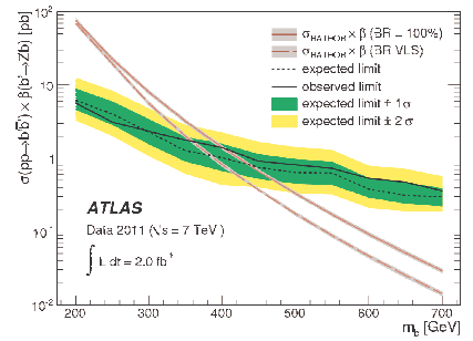
Figure 5: 95% C.L. upper limits on the b'\bar{b}' cross-section as a function of the b' mass, in the Z + b channel.
