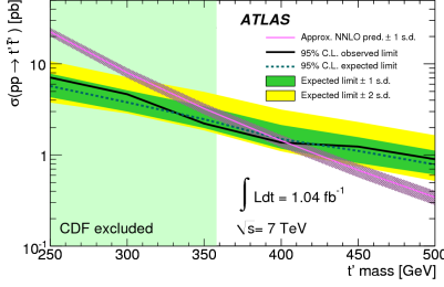
Figure 1: 95% C.L. upper limits on the t'\bar{t}' cross-section as a function of the t' mass, in the lepton+jets channel.
