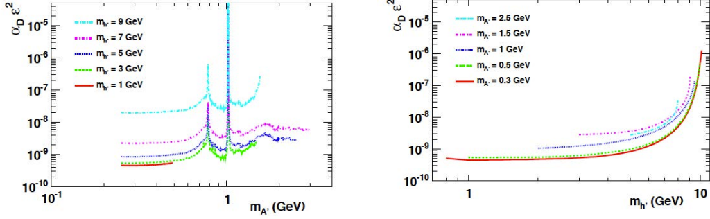
Figure 1: Limits on \alpha_D \epsilon^2 for the Dark Photon (left) and Dark Higgs (right).
