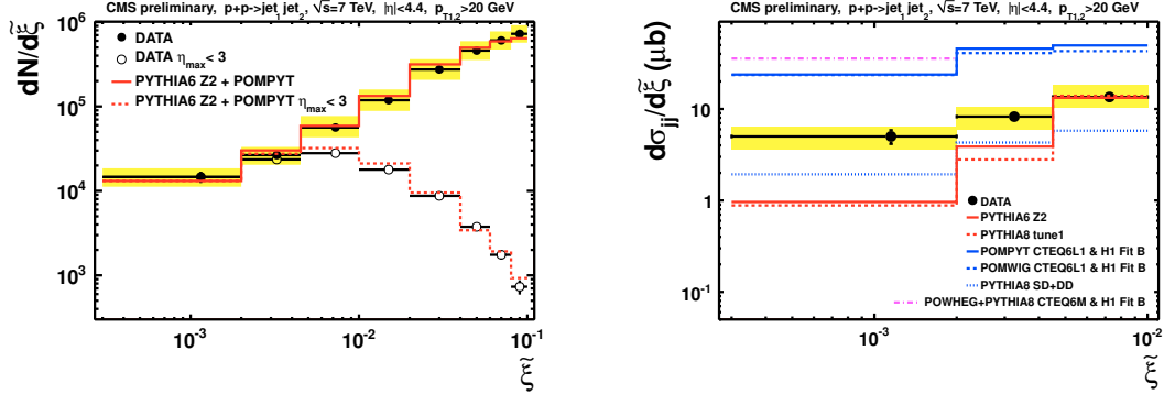
Figure 1: Left: Reconstructed \tilde{\xi} distributions compared to MC predictions including diffractive dijet production (PYTHIA6 + POMPYT) without (solid line) and with (dashed line) the \eta_{\max} < 3 ( \eta_{\min} > -3 ) condition. The MC diffractive dijet contribution has been scaled by a factor of 0.23, obtained from a fit to the data. Right: The differential cross section for dijet production as a function of \tilde{\xi} for jets with -4.4 < \eta < 4.4 and p_T > 20 GeV. The points are plotted at the centre of the bins. The predictions of non-diffractive and diffractive MC generators are also shown (see text). The error bars indicate the statistical uncertainty and the band represents the jet and calorimeter energy-scale uncertainties added in quadrature.
