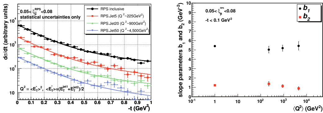
Figure 2: (left) t_{\bar{p}} distributions for SD RPS data of various average Q^2 values within 0.05 < \xi_p^{\text{RPS}} < 0.08 ; (right) the slope parameters b_1 and b_2 vs \langle Q^2 \rangle of a fit to the form dN_{\text{events}}/dt = N_{\text{norm}}(A_1 e^{b_1 t} + A_2 e^{b_2 t}) , with A_2/A_1 = 0.11 (average over all data subsamples). The RPS inclusive points have been placed arbitrarily at \langle Q^2 \rangle = 1 \text{ GeV}^2 .
