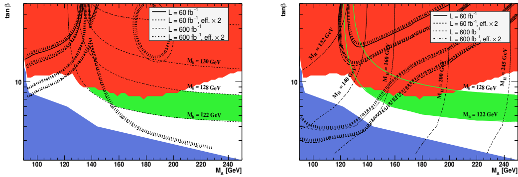
Figure 2: 3\sigma evidence and mass M_h ( M_H ) contours for h(H) \rightarrow b\bar{b} channel in CEP production in the M_A - \tan\beta plane of the MSSM are shown on left (right) within the M_h^{max} benchmark scenario. The results are shown for four assumed effective luminosities (see the text). The lighter (dark) shaded region corresponds to the parameter region excluded by the LEP (Tevatron) Higgs boson searches. The region 122 < M_h < 128 GeV refers to the hypothesis of Higgs bosons found at 125 GeV with assumed theory and experimental uncertainties.
