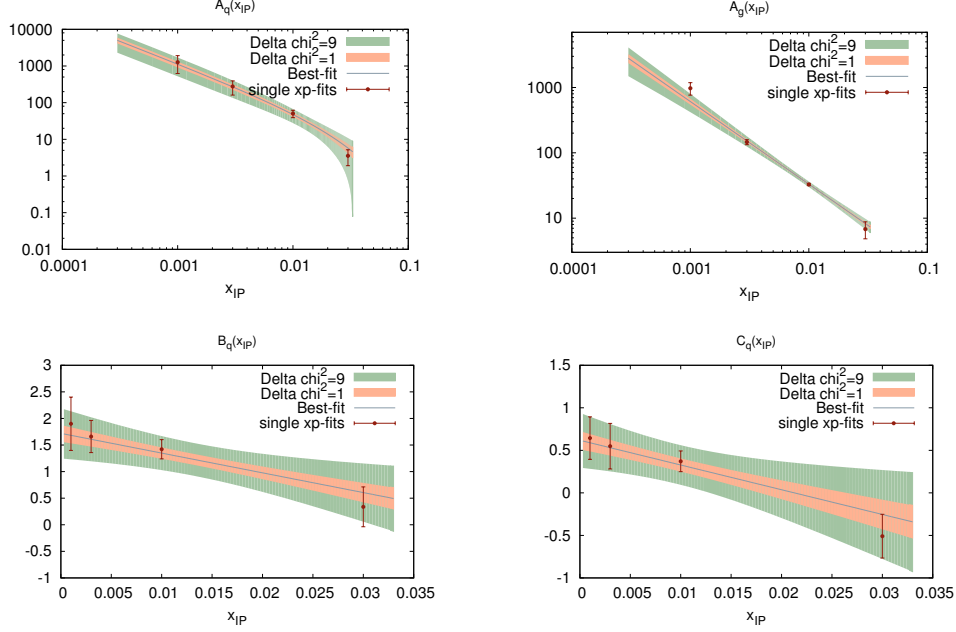
Figure 1: Parameters as a function of x_P . Red dots are the results from pQCD fits at fixed x_P . The grey line are best-fit prediction from x_P -combined fit. The bands represent the propagation of experimental uncertainties by using the Hessian method [10].
