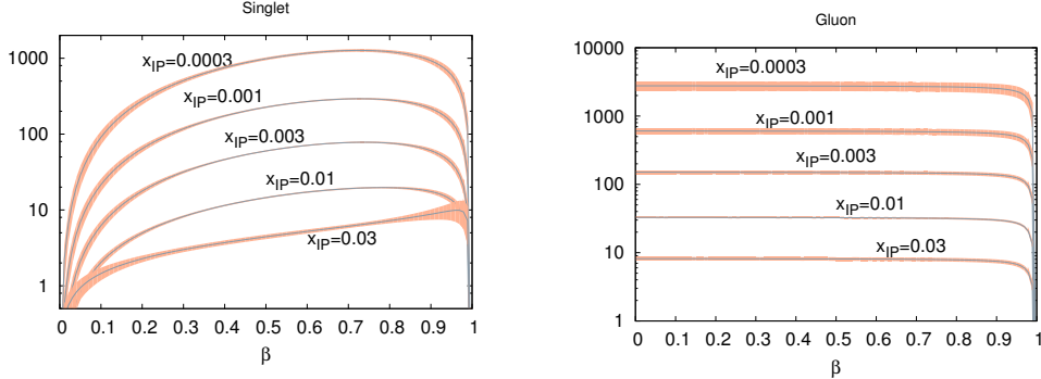
Figure 2: Singlet and gluon initial condition at Q_0^2 as a function of \beta for different x_{\mathcal{P}} -values. The bands represent the propagation of experimental uncertainties by using the Hessian method [10].
