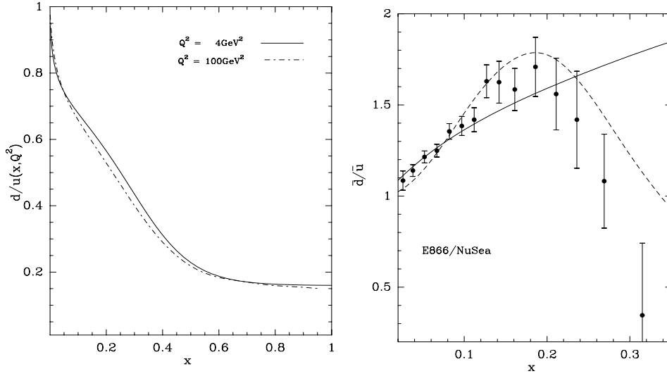
Figure 2: Left : The ratio d(x)/u(x) as function of x for Q^2 = 4 \text{ GeV}^2 (solid line) and Q^2 = 100 \text{ GeV}^2 (dashed-dotted line). Right : Comparison of the data on \bar{d}/\bar{u} versus x , from E866/NuSea at Q^2 = 54 \text{ GeV}^2 [7], with the prediction of the statistical model (solid curve) and the set 1 of the parametrization proposed in Ref. [8] (dashed curve).
