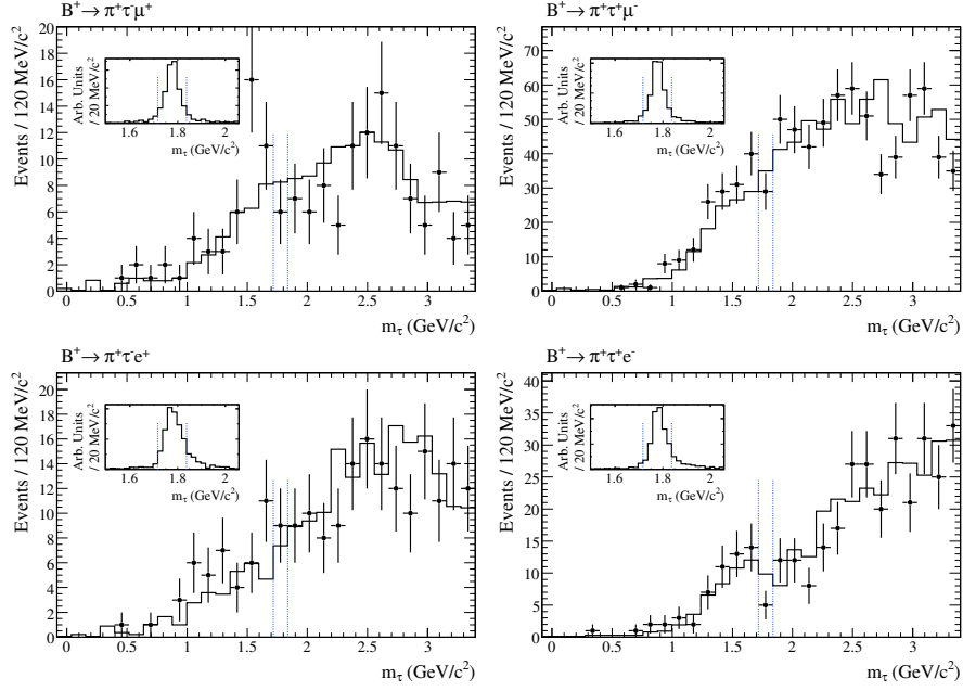
Figure 2: Observed distributions of the \tau invariant mass for the B \rightarrow \pi\tau\ell modes. The distributions show the sum of the three \tau channels ( e, \mu, \pi ). The points with error bars are the data. The solid line is the background MC which has been normalized to the area of the data distribution. The dashed vertical lines indicate the m_\tau signal window range. The inset shows the m_\tau distribution for signal MC.
