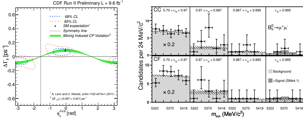
Figure 1: Left: 68% and 95% confidence regions in the plane (\phi_s, \Delta\Gamma_s) from profile-likelihood of CDF data. Right: CDF B_s^0 \rightarrow \mu^+ \mu^- data compared with the expected background, for “Central Central (CC)” and “Central Forward (CF)” muons, according to the detector region.
