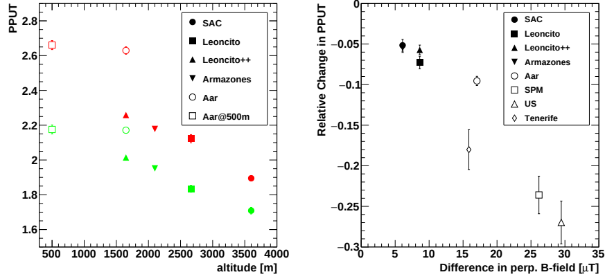
Figure 3: Left: Performance per unit time (PPUT; see text for definition) as function of altitude for the site candidates located in the Southern hemisphere. Red-colored markers indicate results for the arrays pointing in southerly directions, green markers pointings towards the North. Right: Relative difference in PPUT (defined as (PPUT1 - PPUT2) / (0.5 * (PPUT1 + PPUT2)) ) for pairs of simulations at the same site, pointing at 20^\circ zenith angle to the North and the South, versus difference in perpendicular B-field strength between these two directions. Northern and southern site candidates are included in this figure. The differences in the size of the uncertainties is due to the much lower number of MC events simulated for the northern site candidates.
