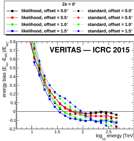
Figure 3: Energy bias for 0° zenith angle.
