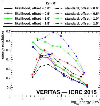
Figure 4: Energy resolution for 0° zenith angle.
