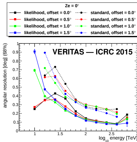
Figure 5: Angular resolution for 0° zenith angle.
