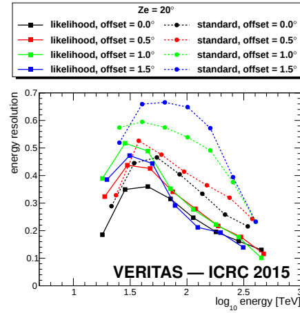
Figure 7: Energy resolution for 20° zenith angle.
