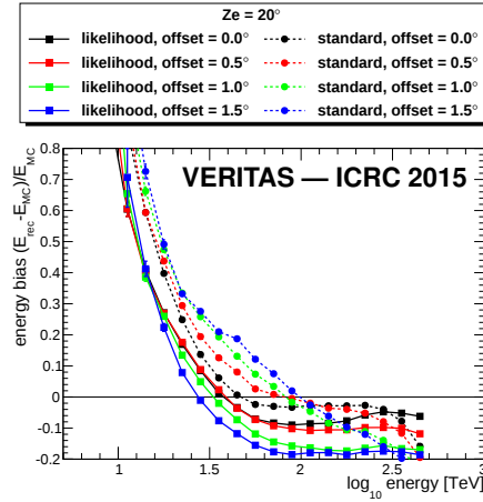
Figure 6: Energy bias for 20° zenith angle.
