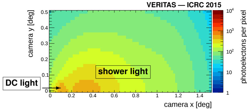
Figure 2: Predicted average light distribution in the camera ( template ) for iron showers with E = 30 TeV, with a distance of 50 m between the detector and shower core, h = 33 km. The origin is defined by the primary particle’s arrival direction. The x-axis is defined by the long image axis. Note the contribution from direct Cherenkov light at around 0.1^\circ from the primary’s direction, clearly distinguishable from the broader contribution from the Cherenkov light emitted by the shower particles.
