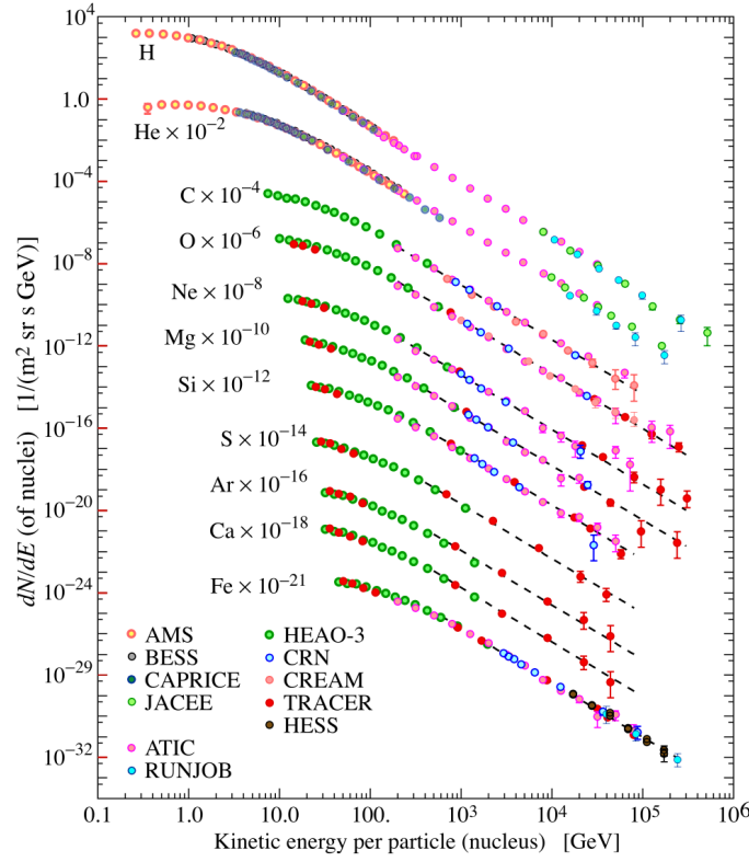
Figure 1: Energy spectra of various elements in cosmic rays, measured by different experiments over a large energy range, from [3].
