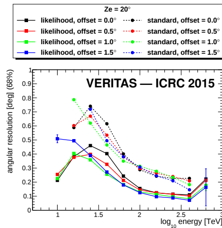
Figure 8: Angular resolution for 20° zenith angle.
