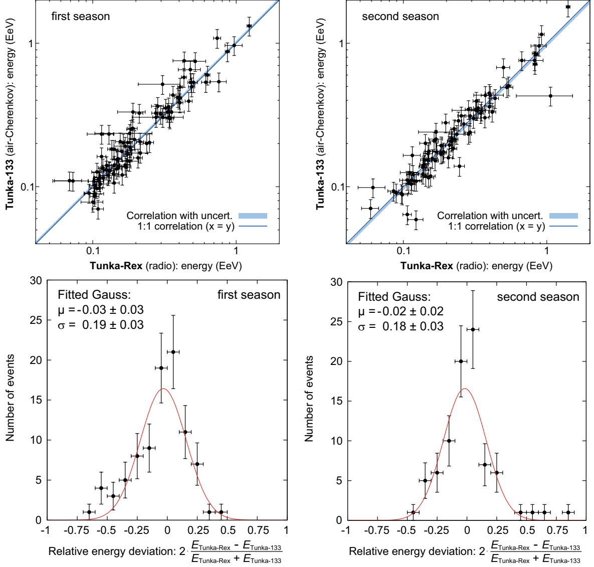
Figure 9. Comparison of the first and second season: reconstructed energy (cf. figure 7).
