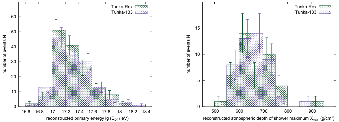
Figure 4. Distributions of energy, E_{\text{pr}} , and atmospheric depth of the shower maximum, X_{\max} , of the Tunka-Rex events used in the present analysis. The figure shows the reconstructed values by both Tunka-Rex and Tunka-133. Bars represent the statistical uncertainty calculated as \sqrt{N} .
