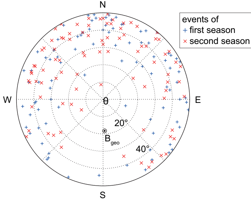
Figure 2. Sky map of the Tunka-Rex events of both seasons. The efficiency rises with zenith angle and is smaller for arrival directions close to the geomagnetic field \mathbf{B}_{\text{geo}} .
