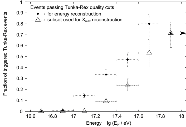
Figure 5. Fraction of events which passes the quality cuts applied for the Tunka-Rex energy and X_{\max} reconstructions, respectively, in comparison with all events triggered by the fully efficient Tunka-133 array in the inner area ( r < 500 m).
