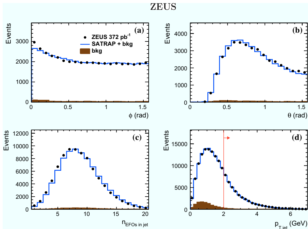
Fig. 6 Comparison between data and MC for variables characterising the jet properties in the \gamma^* -IP rest frame: a the azimuthal angle, \phi , b the polar angle, \theta , c the number of EFOs clustered into a jet and d the jet transverse momentum, p_{T,jet} . Other details as for Fig. 4
