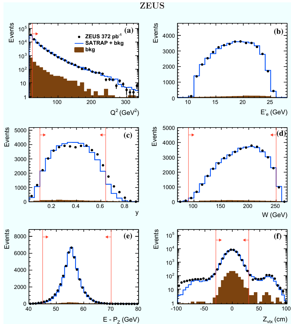
Fig. 4 Comparison between data ( dots ) and the sum ( line ) of the SATRAP MC and background contributions ( shaded ), where events with a dissociated proton are not treated as background, for kinematic variables: a exchanged photon virtuality, Q^2 , b scattered electron energy, E'_e , c inelasticity, y , d invariant mass of the \gamma^*-p system, W , e the quantity E - P_z and f the Z -coordinate of the interaction vertex.
