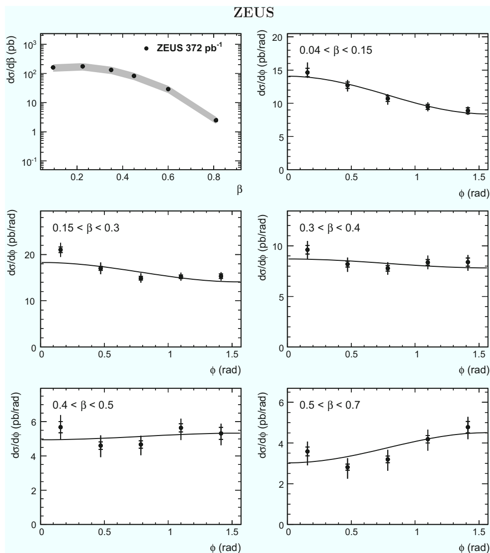
Fig. 11 Differential cross sections for exclusive dijet production: d\sigma/d\beta (in log scale) and d\sigma/d\phi (in linear scale) in five bins of \beta . Contributions from proton-dissociative dijet production were subtracted. The full line represents the fitted function proportional to 1 + A \cos 2\phi . Statistical and systematic uncertainties were included in the fit. The total error bars show statistical and systematic uncertainties added in
