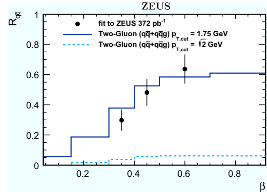
Fig. 16 The R_{q\bar{q}} = \sigma(q\bar{q})/(\sigma(q\bar{q}) + \sigma(q\bar{q}g)) , determined in a fit of the predicted shapes to the measured \phi distributions given in Fig. 11. The fit takes into account the full covariance matrix. The predicted ratio is shown for two choices of p_{T,cut} : for the \sqrt{2} GeV used for the published calculations [17] and for 1.75 GeV, determined in a fit
