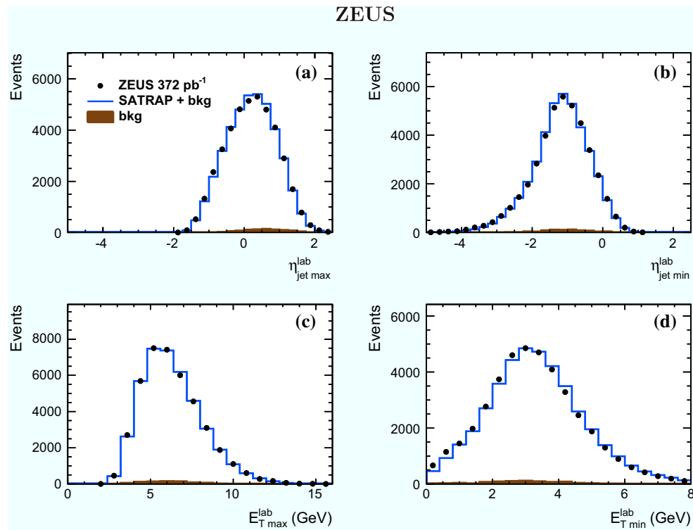
Fig. 7 Comparison between data and MC for variables characterising the properties of the higher and the lower energy jets in the LAB frame: a and b the jet pseudorapidity, c and d the jet transverse energy. Other details as for Fig. 4
