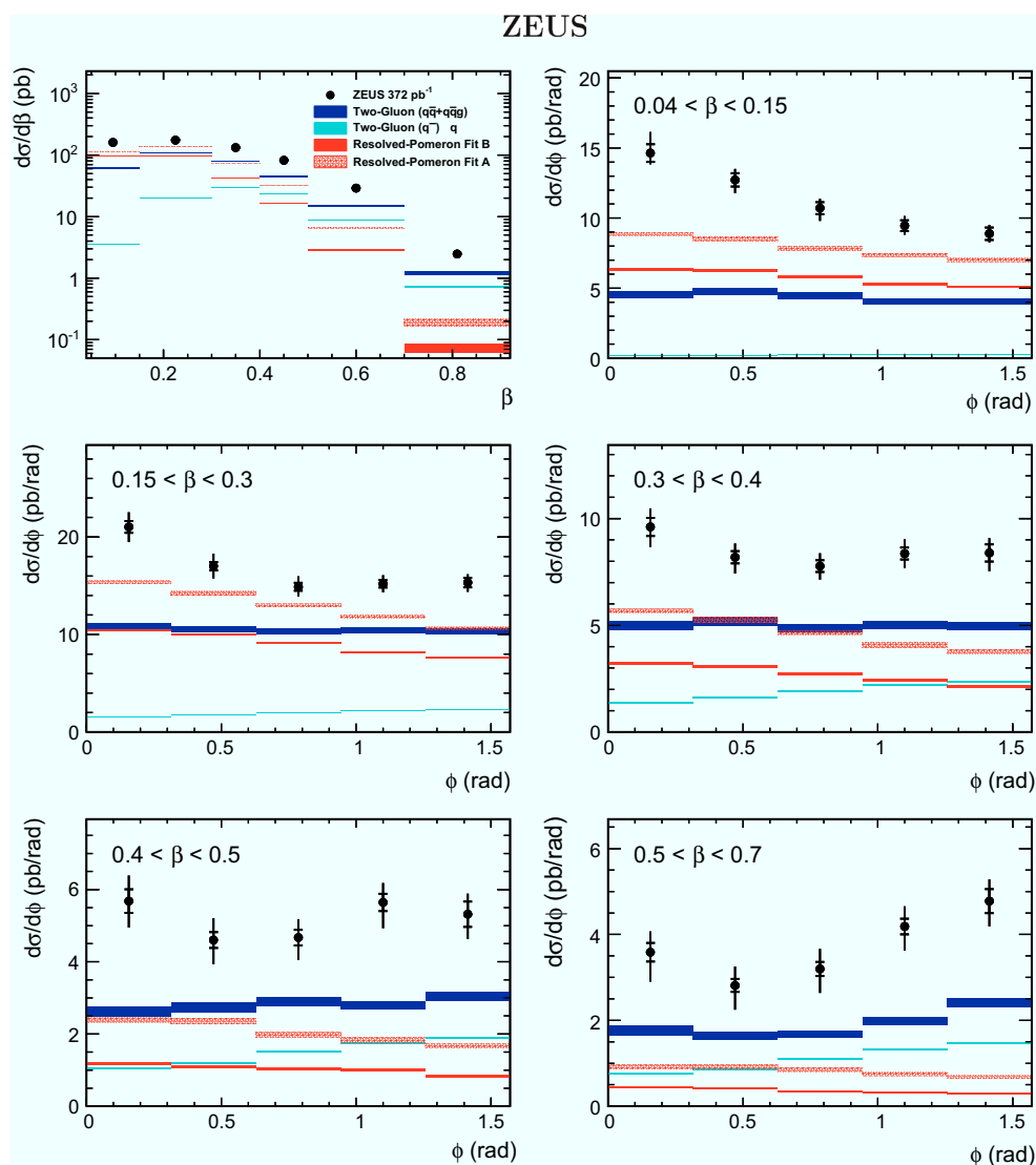
Fig. 17 Differential cross sections as in Fig. 11 in comparison to model predictions d\sigma/d\beta (in log scale) and d\sigma/d\phi in bins of \beta (in linear scale). Contributions from proton-dissociative dijet production were subtracted. The systematic uncertainties do not include the uncertainty
