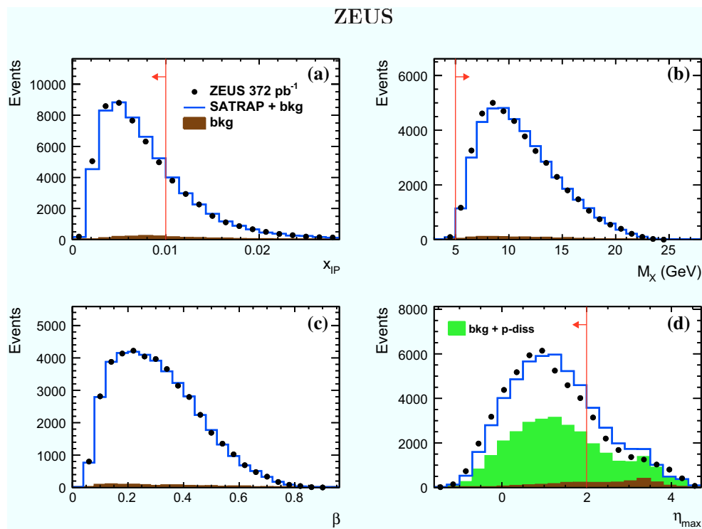
Fig. 5 Comparison between data (dots) and the sum (line) of the SATRAP MC and background contributions (dark histogram), where events with a dissociated proton were not treated as background, for the kinematic variables of the diffractive process: a fraction loss in the longitudinal momentum of the proton, x_{IP} , b the invariant mass of the
