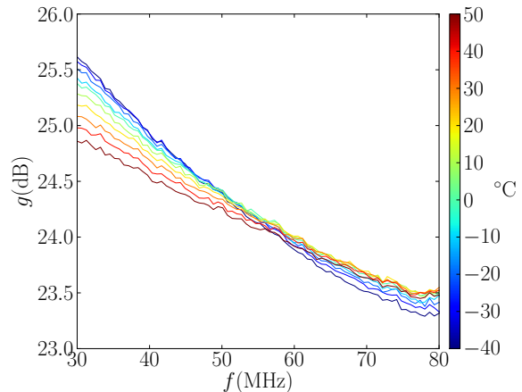
Figure 4. The gain of a LNA at different temperatures. During measurement, i.e., during winter nights we expect temperatures between -35^{\circ}\text{C} and 0^{\circ}\text{C} .
