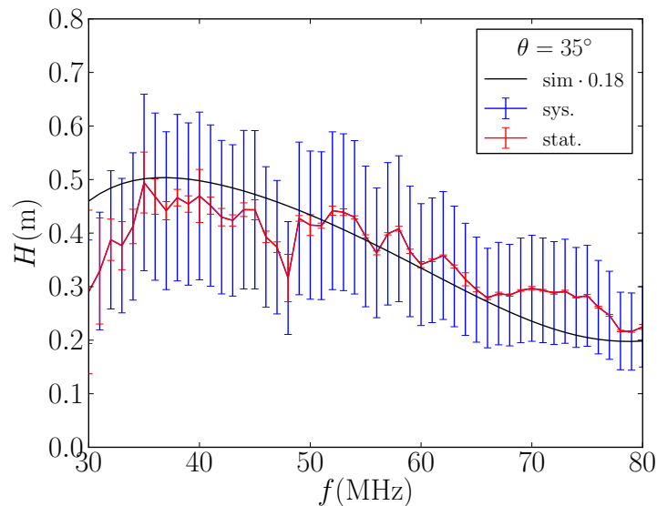
Figure 5. The vector effective length of the SALLA, obtained from the calibration of a Tunka-Rex antenna station and from simulation data. The latter is scaled down for easier comparison.
