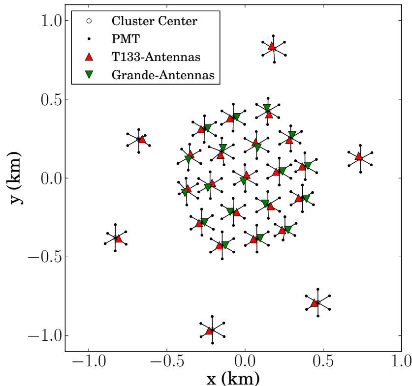
Figure 1. Map of the Tunka-Rex Layout. There is one antenna next to each cluster center of the Tunka-133 PMT stations.
