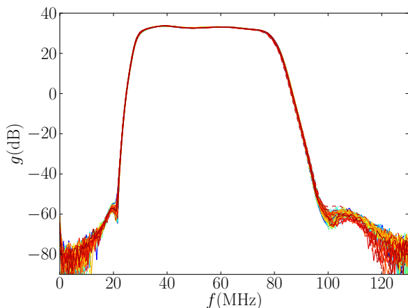
Figure 3. The gain of the filter amplifiers for all 25 filters in different colors.
