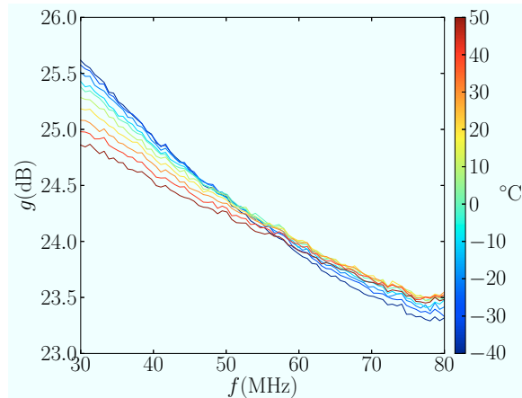
Figure 4. The gain of a LNA at different temperatures. During measurement, i.e., during winter nights we expect temperatures between -35^{\circ}\text{C} and 0^{\circ}\text{C} .
