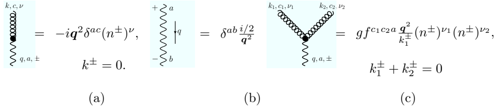
Figure 1: The direct transition vertex (a), the reggeized gluon propagator (b) and the unregulated order g induced vertex (c)
