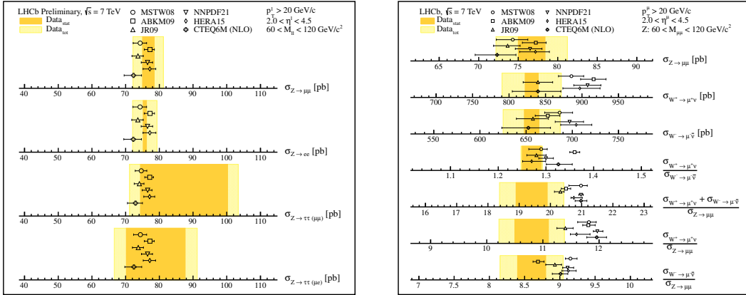
Figure 1: Summary and comparison to theory for the Z cross-section measurements (left) and W and Z cross-section and ratio measurements (right)
