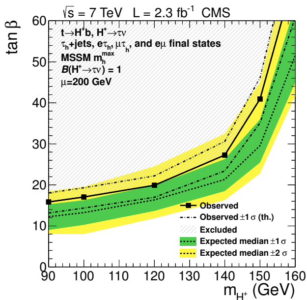
Figure 4: The exclusion region in the M_{H^+} - \tan\beta MSSM parameter space obtained from the combined CMS analysis for the M_{H^+}^{\max} MSSM scenario. The green and yellow bands indicate the corresponding 68% and 95% intervals.
