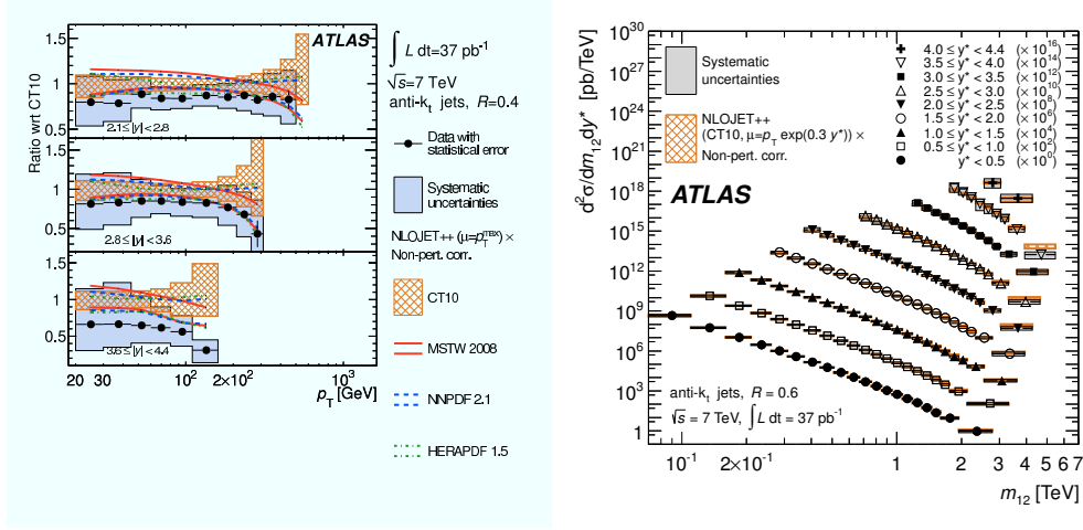
Figure 5: Left: ATLAS data on inclusive jet cross sections as a function of p_t in high rapidity bins. The data are shown in ratio to the predictions of NLOjet++ made using CT10 PDFs, with other PDF predictions shown for comparison. Right: ATLAS di-jet data as a function of di-jet invariant mass in rapidity bins
