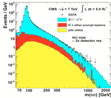
Figure 11: The CMS dielectron invariant mass distribution [23] (left); ATLAS expected and observed 95% CL upper limits on \sigma \times BR as a function of mass for various Z' models ( ee and \mu\mu channels) combined [24].
