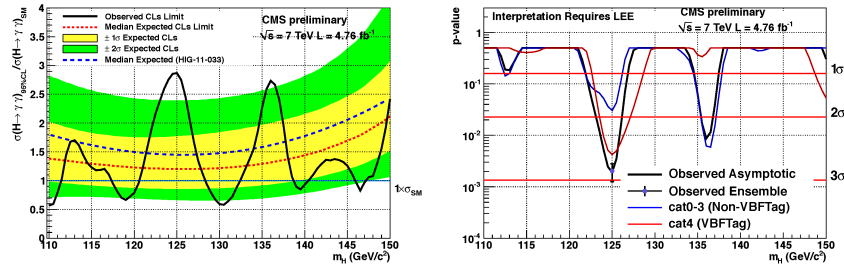
Figure 4: Exclusion limit at 95% CL on the cross section of a SM scalar boson decaying into two photons as a function of the boson mass and relative to the SM cross section, the theoretical uncertainties on the cross section have been included in the limit setting (left); the observed local p-values for the combined event class, the VBF and non-VBF classes (right). From [10].
