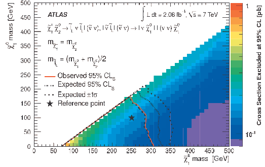
Figure 10: Example of a diagram pour chargino-neutralino production at the LHC (left); observed and expected 95% CL limit contours for chargino and neutralino production in the simplified model scenarios. ATLAS results from [18].
