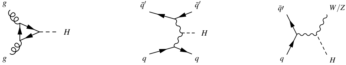
Figure 9: Lowest order Feynman diagrams of the Standard Model Higgs boson production mechanisms exploited by the ATLAS Higgs analyses. Left: Gluon fusion. Middle: Vector boson production. Right: Associated Higgs production.
