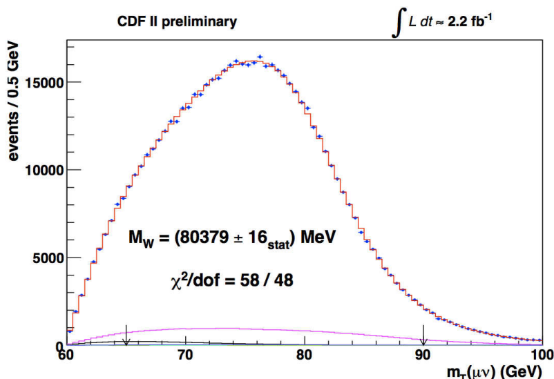
Figure 1: The transverse mass distribution in W \rightarrow \mu\nu events in CDF. The data are compared to the summed signal and background (red histogram) with the background contributions indicated by the lower curves.
