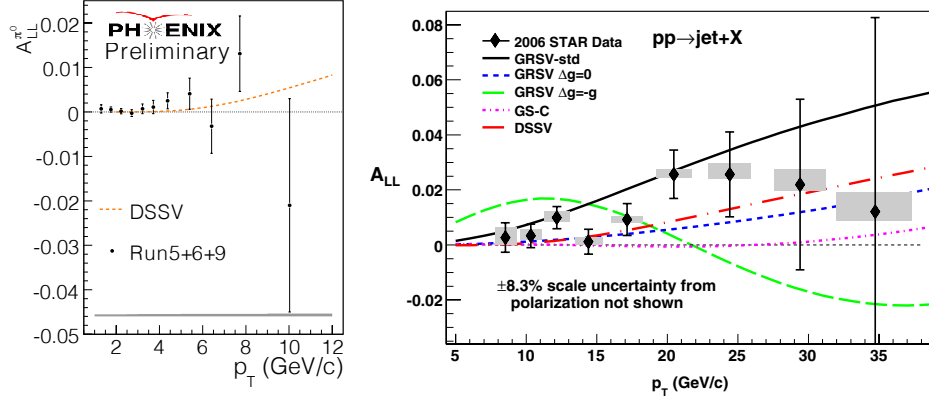
Figure 4: Double spin asymmetries measured at RHIC with \vec{p}\vec{p} collisions at \sqrt{s}=200 GeV compared to DSSV [4]. Left: for \pi^0 production at Phenix [16]; Right: for single jet production at STAR [17].
