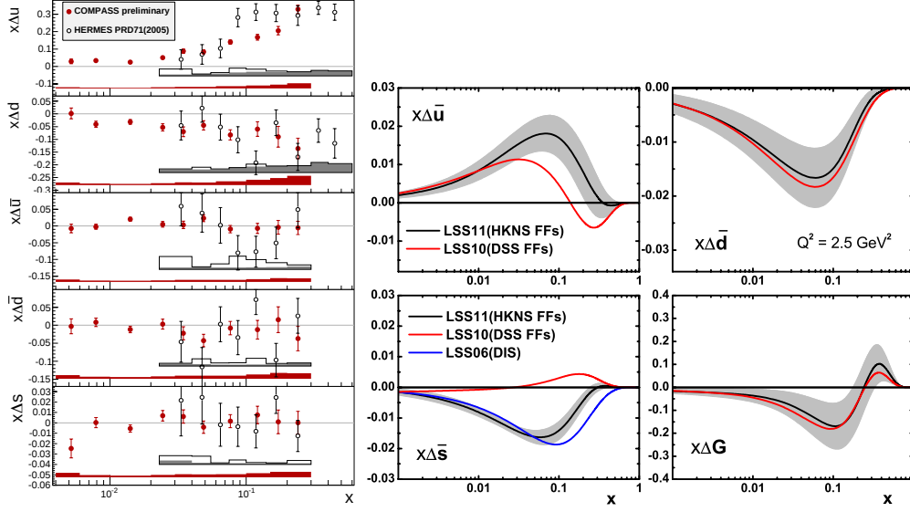
Figure 2: Left: \Delta q(x) measured from SIDIS data at COMPASS [6] and HERMES [7]; Right: Results from global fit [9] using different FF's.
