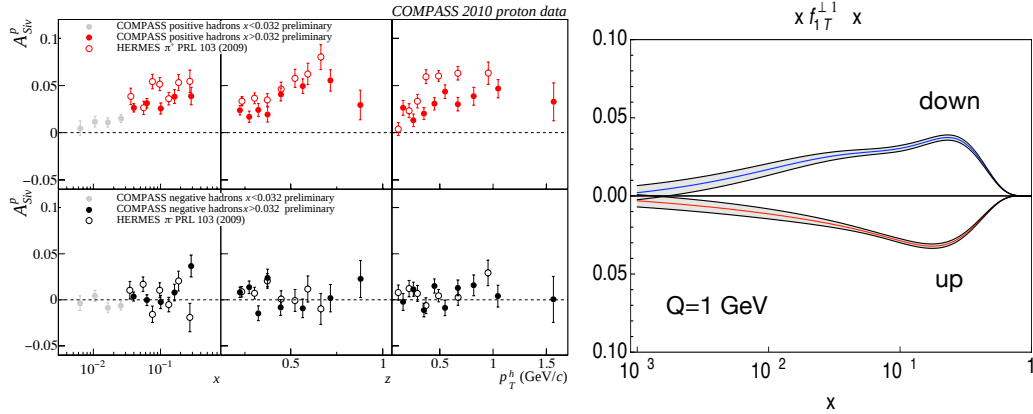
Figure 6: Left: Siverts asymmetry A_{UT}^{sin(\phi_h - \phi_S)} measured on the proton at COMPASS [25] compared to the ones obtained at HERMES [36]; Right: Extracted x.f_{1T}^{\perp} for u and d quarks [39].
