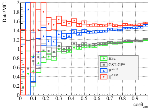
(c) \cos \theta_{\text{zen}} , High-Quality Tracks
