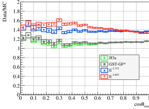
(a) \cos \theta_{\text{zen}} , Trigger Level
