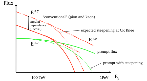
Figure 11: Sketch illustrating the contribution to the single muon spectrum at energies beyond 100 TeV. The “conventional” component from light mesons is sensitive to atmospheric density and varies as a function of the zenith angle [54], that from prompt decays of short-lived hadrons is isotropic. Re-interactions cause the non-prompt spectrum to be steeper. The exact spectral shape depends on the all-nucleon cosmic ray flux, with a significant steepening expected due to the cutoff at the “knee”.
