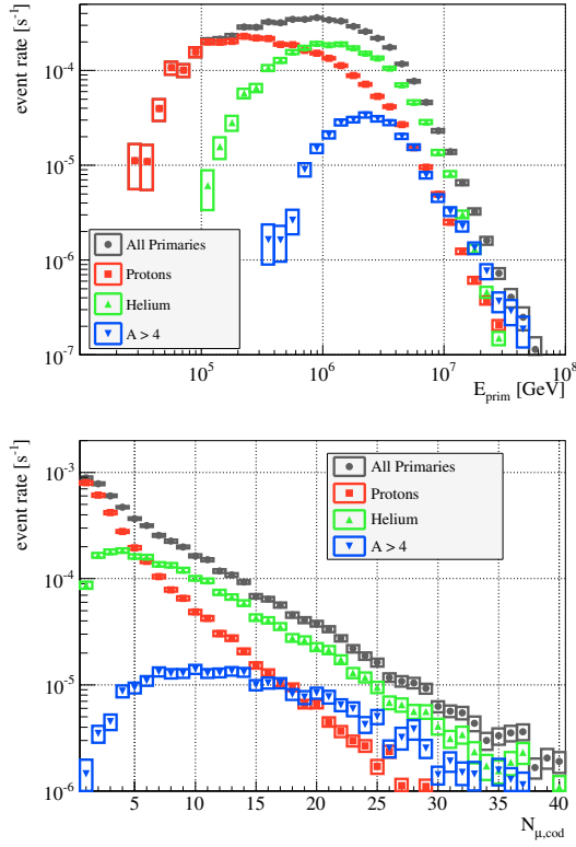
Figure C.2: Parameter distributions separated by primary cosmic ray type for simulated high-energy muon events with reconstructed surface energies between 30 and 50 TeV. True primary energy (top) and muon bundle multiplicity at detector depth (bottom).
