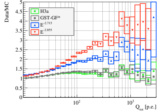
(b) Q_{\text{tot}} , Trigger Level
