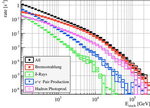
Figure 3: Energy spectra of discrete stochastic energy losses along muon tracks simulated using the mmc code [69]. The data sample corresponds to events with more than 1,000 registered photo-electrons in the IceCube detector. For demonstration purposes, the primary cosmic ray spectrum is modeled as an unbroken E^{-2.7} power law.
