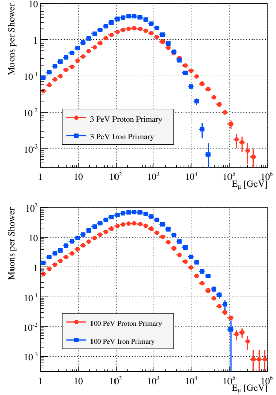
Figure 9: Distribution of muon energies in individual air showers at the IceCube detector depth simulated with CORSIKA/SIBYLL [12, 65], averaged over all angles. Top: E_{\text{prim}} = 3 \text{ PeV} . Bottom: E_{\text{prim}} = 100 \text{ PeV} . The threshold effect visible at high muon energies in the top plot is due to the lower energy per nucleon in iron primaries. As the total energy increases, this effect becomes less and less visible and the spectra are identical except for a scaling factor.
