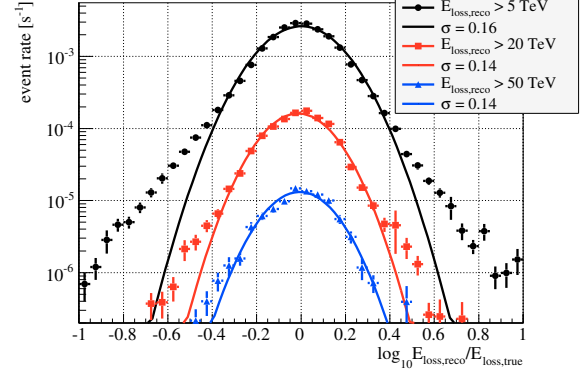
Figure A.4: Ratio between reconstructed and true shower energy for simulated events weighted to an E^{-2.7} power-law primary cosmic ray flux spectrum. Around the peak the distribution can be closely approximated by a Gaussian distribution with a width varying between approximately 0.16 and 0.14.
