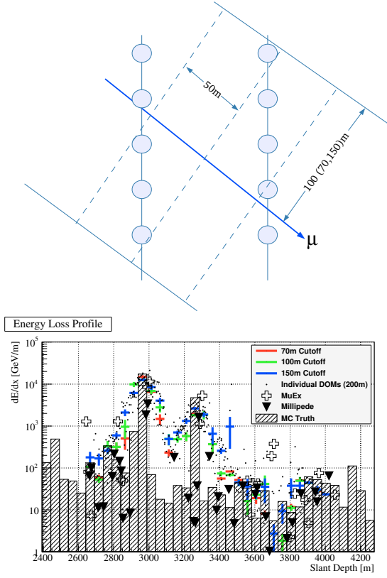
Figure A.3: Top: Construction of differential energy deposition estimator. DOMs are represented by circles. The maximum lateral distance from the track up to which individual data points are included in the reconstruction can be varied depending on specific requirements. Bottom: Comparison between true and reconstructed energy loss in simulated event with parameters: E_{\text{shower, reco}} = 1165 TeV (True Value: 852 TeV), \cos \theta_{\text{zen, reco}} = 0.556 (True Value: 0.551) E_{\mu, \text{reco}} = 2493 TeV (True Value: 1854 TeV). The shower energy corresponds to the highest single stochastic loss at approximately 3000 m slant depth. Reconstructions using two different likelihood methods [64] are shown for comparison.
