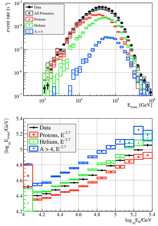
Figure C.3: Top: Truncated Energy observable in CORSIKA simulation weighted to GST-Global Fit flux and experimental data. Event selection criteria are the same as in Fig. C.2. Bottom: Mean Truncated Energy observable in dependence of reconstructed leading muon surface energy for simulated and experimental data.
