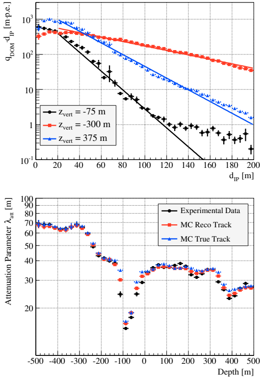
Figure A.2: Top: Lateral attenuation of photon intensity along muon bundle tracks in experimental data. The vertical depth ranges, corresponding to DOM position relative to the center of the detector 1949 m below the surface, were chosen to illustrate the strongly varying optical properties of the ice. Bottom: Effective attenuation parameter \lambda_{\text{att}} derived from exponential fit to the data distribution. Experimental values are compared to Monte-Carlo simulation using reconstructed and true track parameters for calculation of the impact parameter d_{\text{IP}} .
