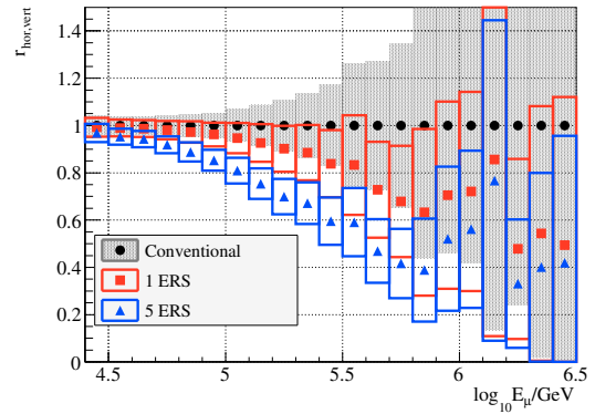
Figure 27: Ratio parameter r_{\text{hor,vert}} expressing deviation of angular distribution from purely conventional flux for various prompt levels in simulation. The size of the error bars corresponds to the statistical uncertainty due to limited availability of simulated data.
