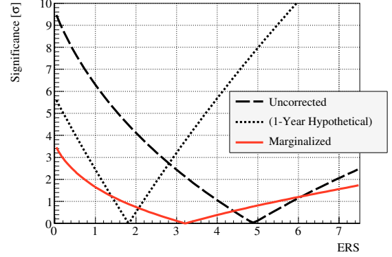
Figure 30: Significance of prompt flux measurement based on angular information. The individual curves correspond to different assumptions about systematic effects as described in the text. Also shown is the hypothetical result which could be achieved with one year of experimental data given unlimited availability of simulated events, assuming a best fit value of 1.8 ERS consistent with theoretical predictions for inclusive prompt muon flux.
