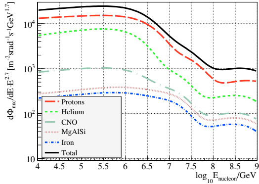
(c) Nucleon Energy E_{\text{nuc}}
