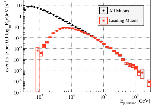
Figure 10: Surface energy distribution for all and most energetic (“leading”) muons in simulated events with a total of more than 1,000 registered photo-electrons in IceCube.
