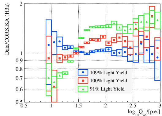
Figure 5: Top: Simulated distributions of total number of photo-electrons in event, separated in dependence of number of muons in bundle at closest approach to the center of the IceCube detector. The functional dependence of the fit is described in the text. Bottom: Change of data/simulation ratio for different assumptions about the light yield, effectively corresponding to the relation between energy deposition and number of registered photo-electrons. The simulation was weighted according to the H3a primary flux model.
