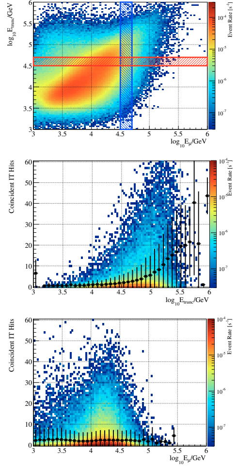
Figure C.1: Top: Reconstructed muon surface energy and truncated mean [63] for experimental data. The sample corresponds to tracks with reconstructed angle within 37 degrees from zenith ( \cos \theta_{zen} > 0.8 ) in selection described in 7, before exclusion of events with shower energies below 5 TeV. Red and blue boxes illustrate selection of data with approximately constant energy measurement. Middle: Number of IceTop tanks registering a signal in coincidence with muon track for fixed reconstructed muon surface energy (blue box). Bottom: Same for fixed truncated mean (red box).
