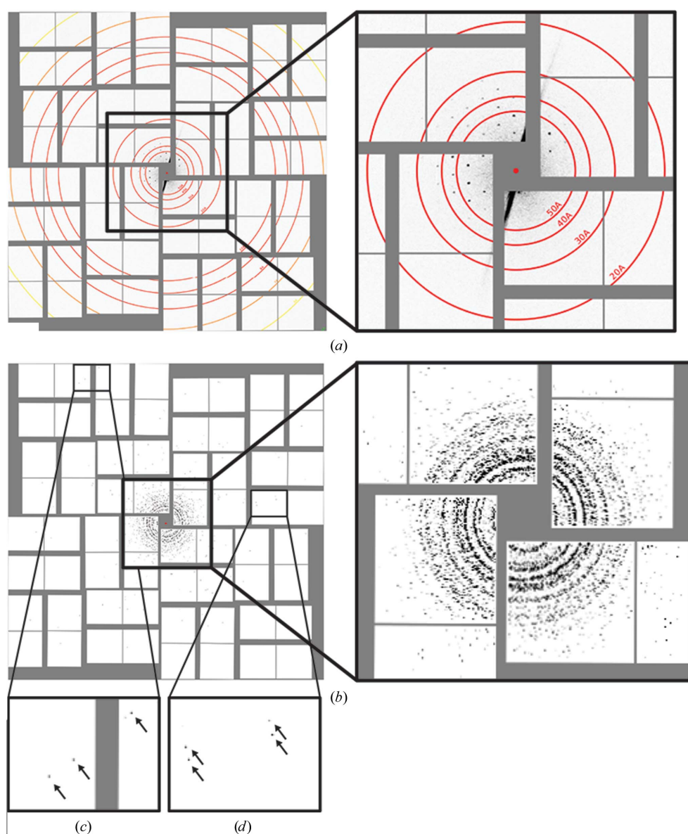
Figure 3 ( a ) Example SFX diffraction image of \Delta PEX11 cells displaying Bragg-sampled reflections with intensities above the background level. ( b ) Composite XRPD patterns assembled from individual diffraction images show that most crystallites diffract to approximately 30 Å resolution, with several crystals displaying diffraction out to the detector edge (6 Å) and corners (5.6 Å) as indicated by arrows in insets ( c ) and ( d ).
