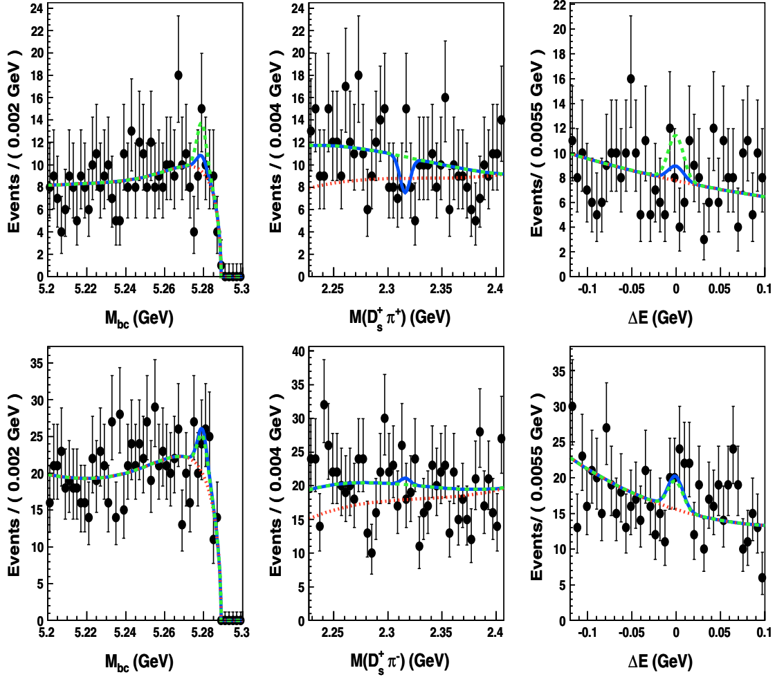
FIG. 7 (color online). The M_{bc} (left), M(D_s^+ \pi) (center) and \Delta E (right) distributions for selected B^+ \rightarrow D^- D_s^+ \pi^+ \pi^+ (top) and B^0 \rightarrow \bar{D}^0 D_s^+ \pi^- (bottom) event candidates for the fit with the signal peak mass restricted to a 5 MeV region centered at M(D_s^+ \pi) = 2317.8 MeV. In the lower plots, the \bar{D}^0 \rightarrow K^+ \pi^- and K^+ \pi^+ \pi^- \pi^- samples are combined. (See text for curves.)
