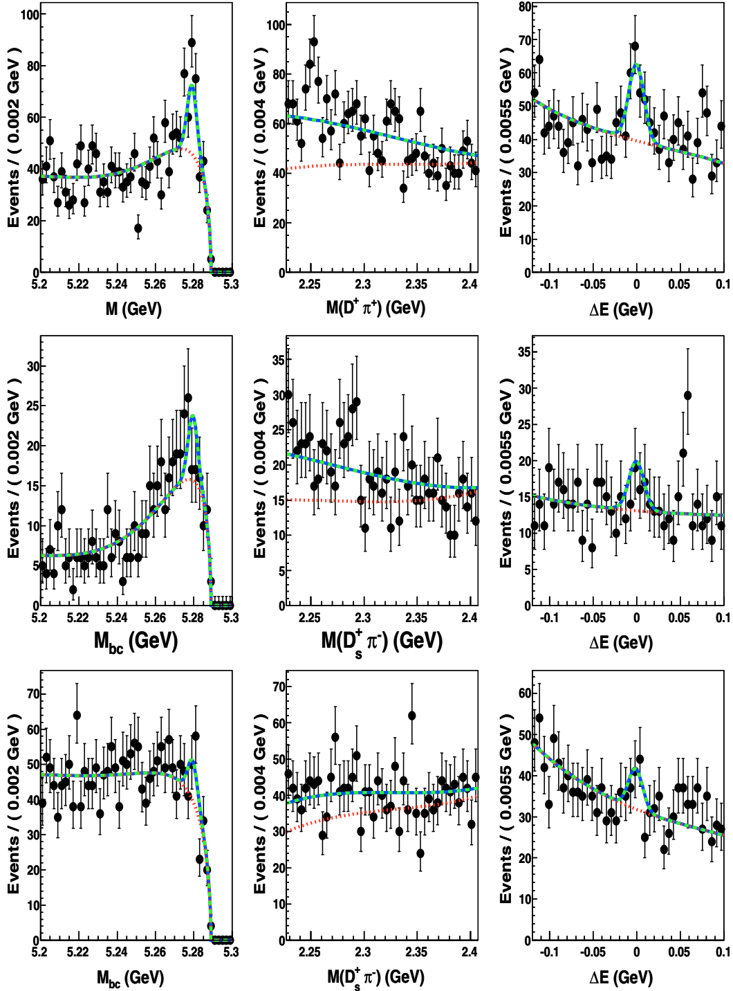
FIG. 6 (color online). The M_{bc} (left), M(D_s^+ \pi) (center) and \Delta E (right) distributions for generic-MC events that pass the D^- D_s^+ \pi^+ (top), \bar{D}^0 D_s^+ \pi^- , \bar{D}^0 \rightarrow K^+ \pi^- (middle) and \bar{D}^0 D_s^+ \pi^- , \bar{D}^0 \rightarrow K^+ \pi^+ \pi^- \pi^- (bottom) channels. The curves are the results of fits described in the text.
