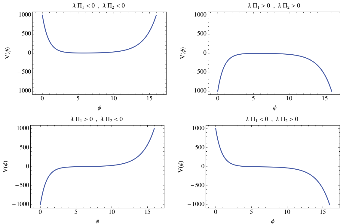
Figure 1. Scalar potential of eq. (3.15) (in units of g_s^2 \left(\frac{W_0}{V}\right)^4 ) for different choices of the topological integers \Pi_1 and \Pi_2 .
