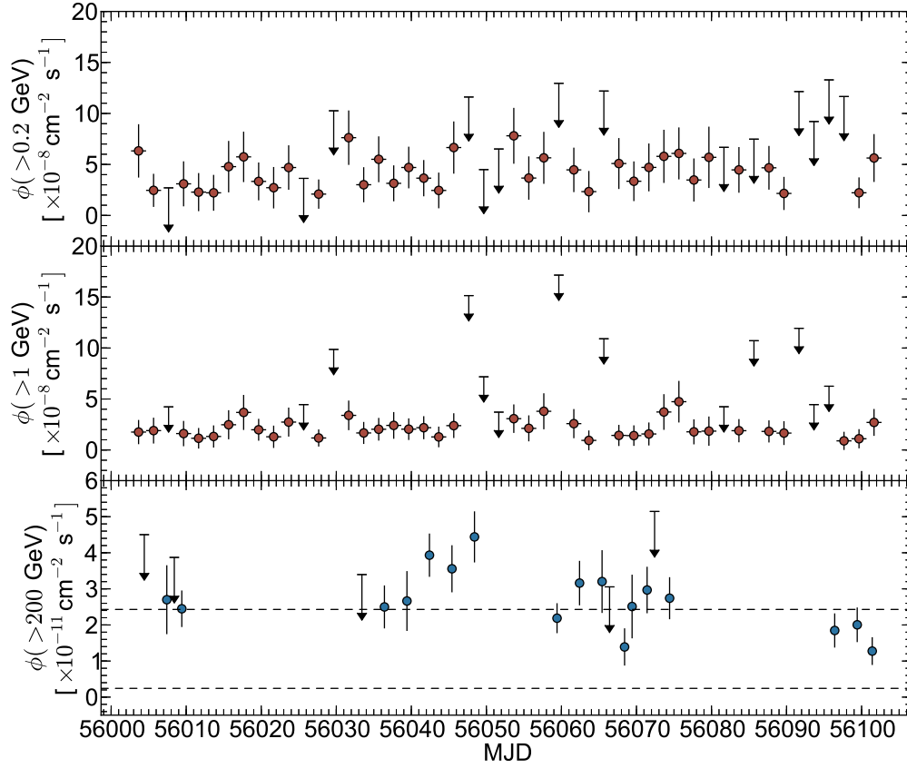
Figure 5. Fermi -LAT PG 1553+113 bi-daily flux light curve (2012) above 200 MeV (upper plot) and 1 GeV (middle plot), in units of \text{cm}^{-2} \text{ s}^{-1} , for the time periods contemporaneous with VERITAS observations, and VERITAS daily integral flux light curve above 200 GeV (lower plot), in units of \text{cm}^{-2} \text{ s}^{-1} . The upper and lower dashed lines indicate the integral fluxes above 200 GeV corresponding to 10% and 1% of the Crab Nebula flux, respectively. The black arrows represent 2\sigma upper limits.
