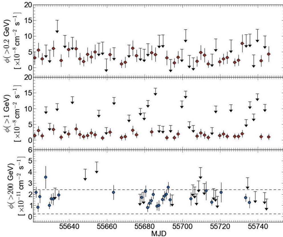
Figure 4. Fermi -LAT PG 1553+113 bi-daily flux light curve (2011) above 200 MeV (upper plot) and 1 GeV (middle plot), in units of \text{cm}^{-2} \text{s}^{-1} , for the time periods contemporaneous with VERITAS observations, and VERITAS daily integral flux light curve above 200 GeV (lower plot), in units of \text{cm}^{-2} \text{s}^{-1} . The upper and lower dashed lines indicate the integral fluxes above 200 GeV corresponding to 10% and 1% of the Crab Nebula flux, respectively. The black arrows represent 2\sigma upper limits.
