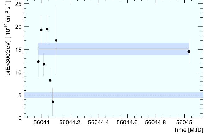
Figure 2. H.E.S.S. light curve of PG 1553+113 during the two nights of the flare period. The continuous line is the measured flux during the flare period while the dashed one corresponds to the pre-flare period (see Table 2 for the flux values). Gray areas are the 1\sigma errors.
