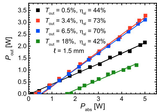
Fig. 2. Laser characteristics and linear fits (straight lines) of an OPSSL-pumped 1.5-mm Yb(5.4%):CALGO crystal. The cw laser output power P_{\text{out}} is plotted against the absorbed pump power P_{\text{abs}} for different output coupler transmissions T_{\text{out}} .
