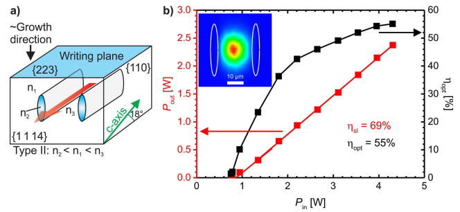
Fig. 4. (a) Schematic of the orientation of waveguide laser crystal. (b) Characteristics of the waveguide laser with the mode-profile measured at 96 mW as inset. The cw output power P_{out} and optical efficiency \eta_{opt} are plotted against the incident power P_{in} .
