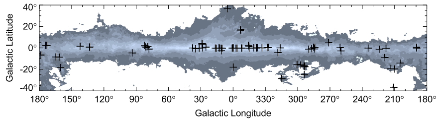
Figure 14. Locations of the \gamma sources in the 3FGL catalog overlaid on a grayscale representation of the model for the Galactic diffuse \gamma -ray emission used for the 3FGL analysis (see Section 2.3). The plotted symbols are centered on the locations of the sources. The model diffuse intensity is shown for 1 GeV, and the spacing of the levels is logarithmic from 1% to 100% of the peak intensity.
