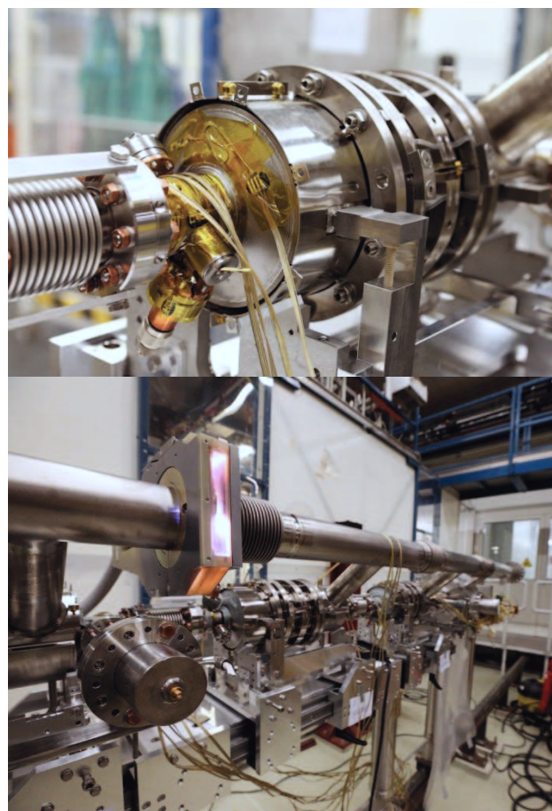
Figure 2: Top: Assembly of the magnetic shielding, blade tuner mechanism and T sensors on the cavity. Bottom: welding operation on the 2 phase line.
