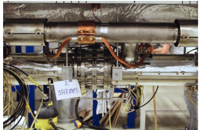
Figure 4: One cavity of the string, after installation of the magnetic shield interconnections between the cavity, the installation of all RF cabling and thermalization braids for the tuner motor and HOM feedthroughs. Motor cables are thermalized on the magnetic shield surfaces.
