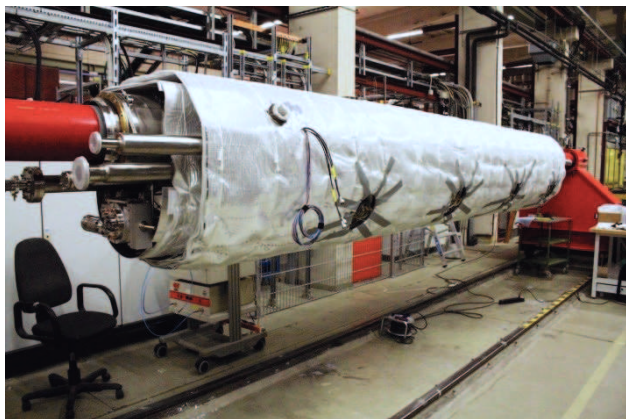
Figure 5: The Module after the installation of the two thermal shields and the cutout of the coupler ports on the MLI blankets.
