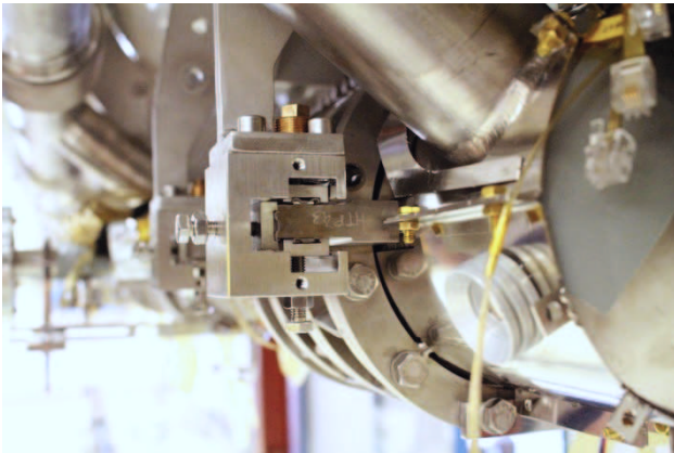
Figure 3: The cavity spring-loaded, roller bearing suspension system.
