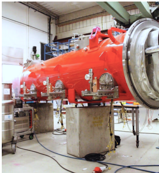
Figure 6: The X3M1 during Warm Coupler parts installation.
