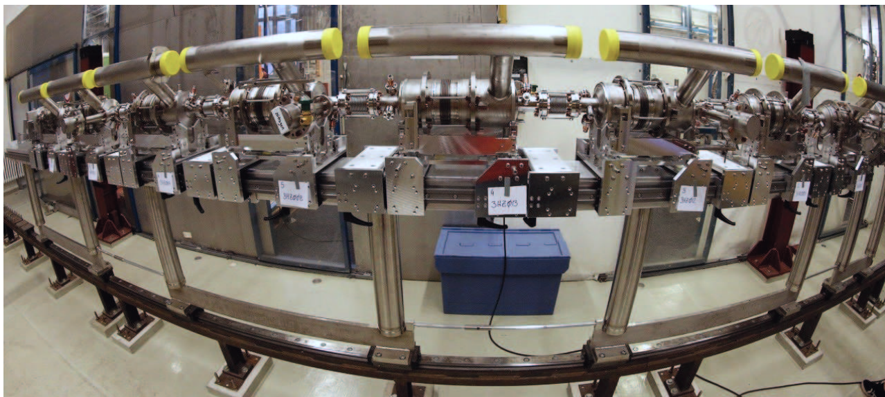
Figure 1: X3M1 string after roll-out from the clean room, supported on the girder.
