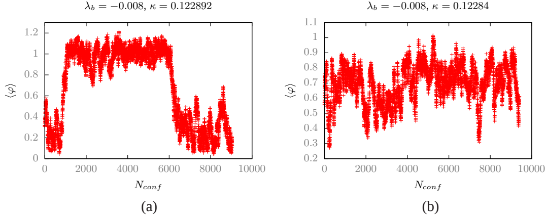
Figure 3: The Monte-Carlo time evolution of \langle \phi \rangle near phase transitions at (a) \kappa = 0.122892 and the lattice volume 20^3 \times 4 , (b) \kappa = 0.12284 and the lattice volume 20^3 \times 6 .
