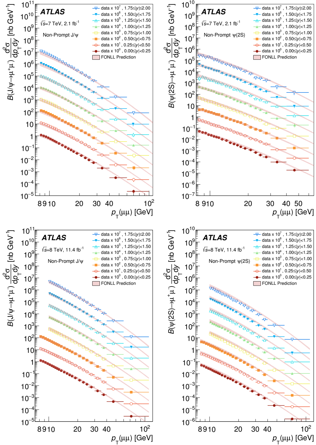
Figure 8: The differential non-prompt cross-section times dimuon branching fraction of J/\psi (left) and \psi(2S) (right) as a function of p_T(\mu\mu) for each slice of rapidity. The top (bottom) row shows the 7 TeV (8 TeV) results. For each increasing rapidity slice, an additional scaling factor of 10 is applied to the plotted points for visual clarity. The centre of each bin on the horizontal axis represents the mean of the weighted p_T distribution. The horizontal error bars represent the range of p_T for the bin, and the vertical error bar covers the statistical and systematic uncertainty (with the same multiplicative scaling applied). The FONLL theory predictions are also shown.
