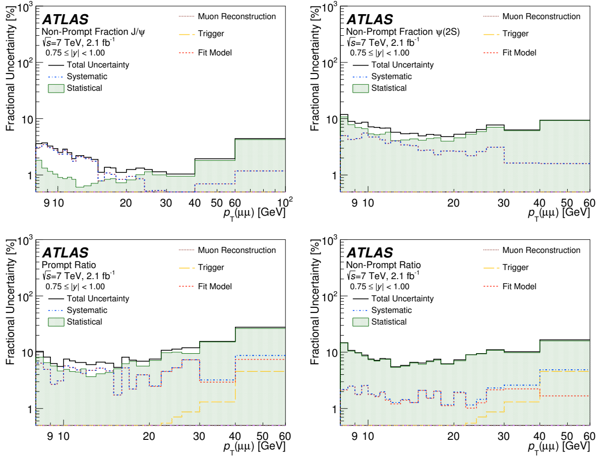
Figure 6: Breakdown of the contributions to the fractional uncertainty on the non-prompt fractions for J/\psi (top left) and \psi(2S) (top right), and the prompt (bottom left) and non-prompt (bottom right) ratios for 7 TeV, shown for the region 0.75 < |y| < 1.00 .
