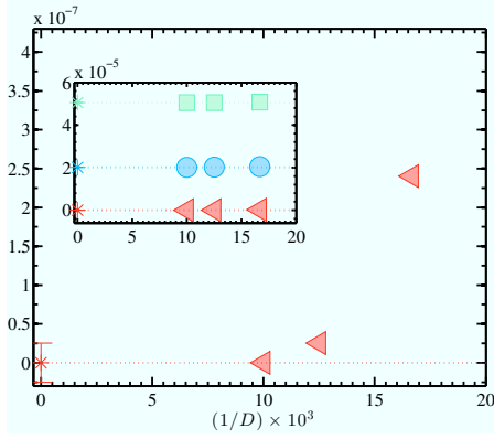
Figure 1: D -dependence of the chiral condensate for \delta = 5 \cdot 10^{-4} (red), 7 \cdot 10^{-4} (blue), 10^{-3} (green) at N = 40 , x = 6.25 and g\beta = 0.4 .
