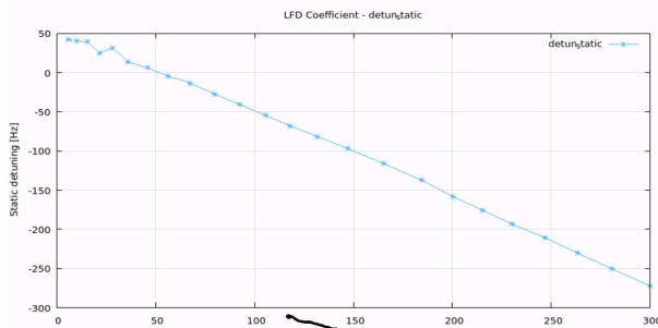
Figure 3: Static detuning change measured in function of cavity gradient.
