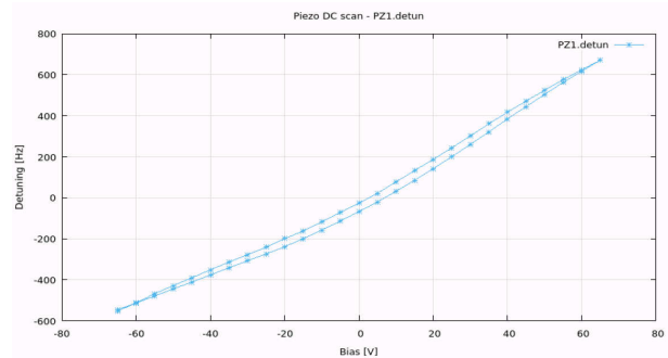
Figure 1: Piezo element tuning range characterization example (XFEL module XM51, cavity 3).
