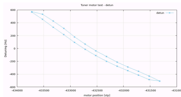
Figure 2: Slow tuner motor behavior characterization (XFEL module XM51, cavity 3).
