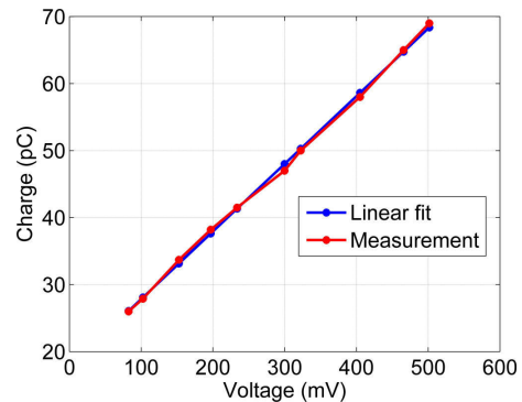
Figure 5: Characteristic of the bunch charge detection subsystem.
