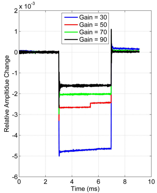
Figure 1: Response of a LLRF system using only a PI feedback controller to a beam pulse.
