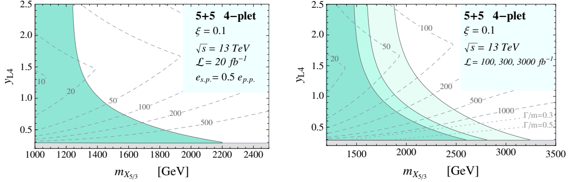
Figure 8: Estimated exclusion on the 5+5 model with only a composite 4-plet for the 13 TeV LHC run. The results are shown in the (m_{X_{5/3}}, y_{L4}) plane for the choice \xi = 0.1 . On the left panel, the green area shows the excluded region for \mathcal{L} = 20 \text{ fb}^{-1} integrated luminosity under the assumption that the signal efficiency of single production processes is 50% of to the pair production one, e_{s.p.} = 0.5 e_{p.p.} . On the right panel the green areas show the expected exclusions for \mathcal{L} = 100, 300, 3000 \text{ fb}^{-1} integrated luminosity (assuming e_{s.p.} = 0.5 e_{p.p.} ). The dotted contours denote the regions with \Gamma(X_{5/3})/m_{X_{5/3}} = 0.3, 0.5 . On both panels the dashed contours show the amount of tuning \Delta estimated by using eq. (3.9).
