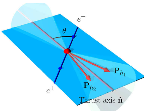
FIG. 2 (color online). Illustration of dihadron fragmentation where the final-state hadrons are depicted as red arrows, the incoming leptons as blue arrows and the event plane—spanned by leptons and initial quarks/thrust axis—is depicted as a light blue plane. In this case, both hadrons are found in the same hemisphere as defined by the thrust axis, and generally out of the plane, as indicated by the cones.
