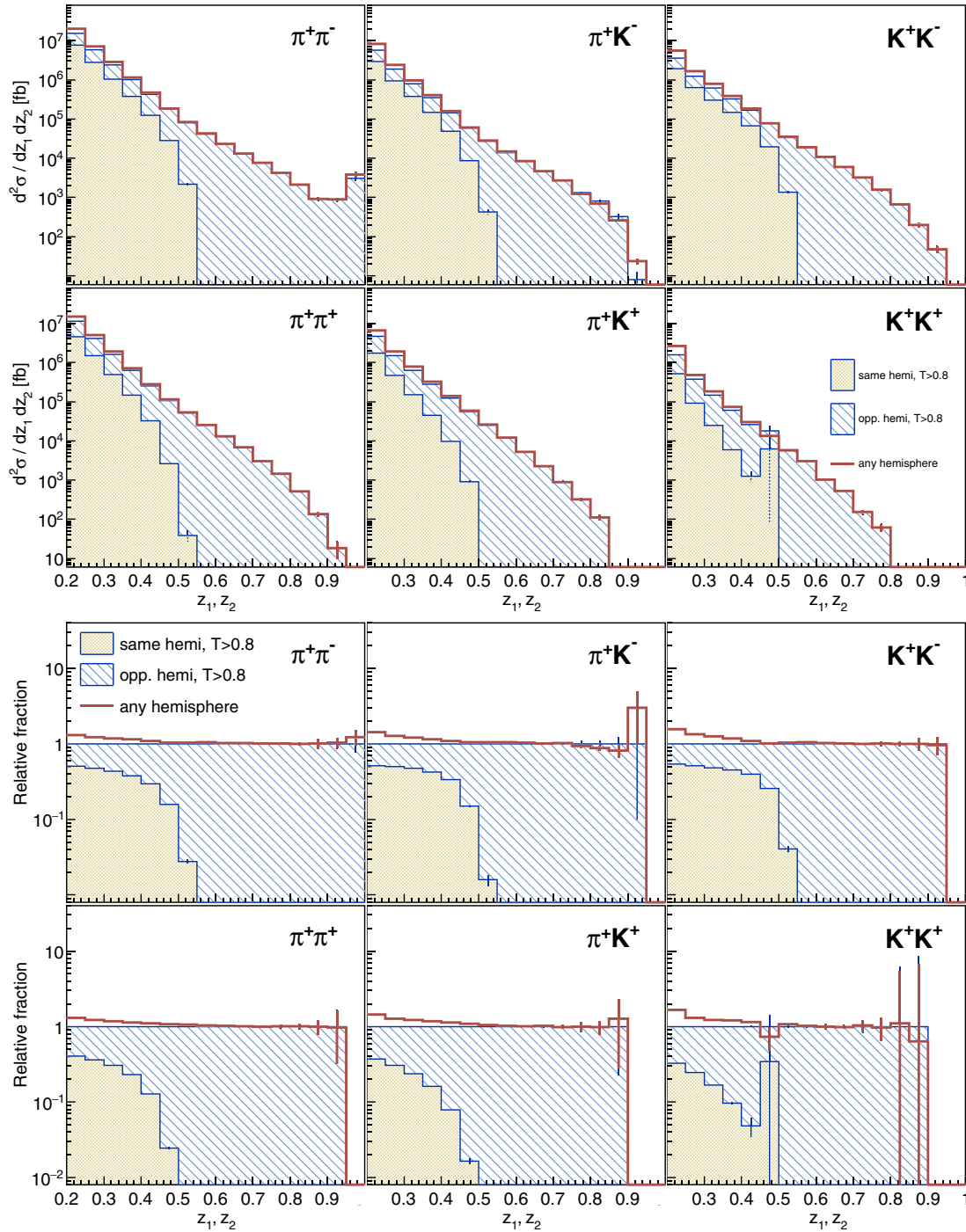
FIG. 17 (color online). Differential cross sections (top panels) and ratios to the same and opposite topology sum (bottom panels) for the main hadron combinations, stacking same (gray filled areas, including thrust selection T > 0.8 ) and opposite (blue hatched areas, including thrust selection T > 0.8 ) hemisphere data and comparing to those without hemisphere assignment (red curves). For visibility, only the diagonal (z_1, z_2) bins and statistical uncertainties are displayed.
