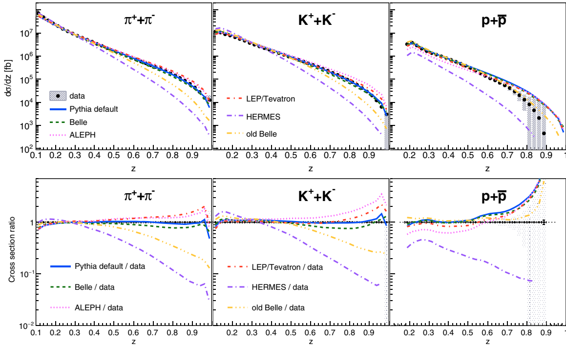
FIG. 23 (color online). Differential cross sections (top panels) and ratios to the data (bottom panels) for the main single hadrons as a function of z . Various MC tunes are also displayed as described in the text. For comparison, the relative statistical and systematic uncertainties are shown for the data as well.
