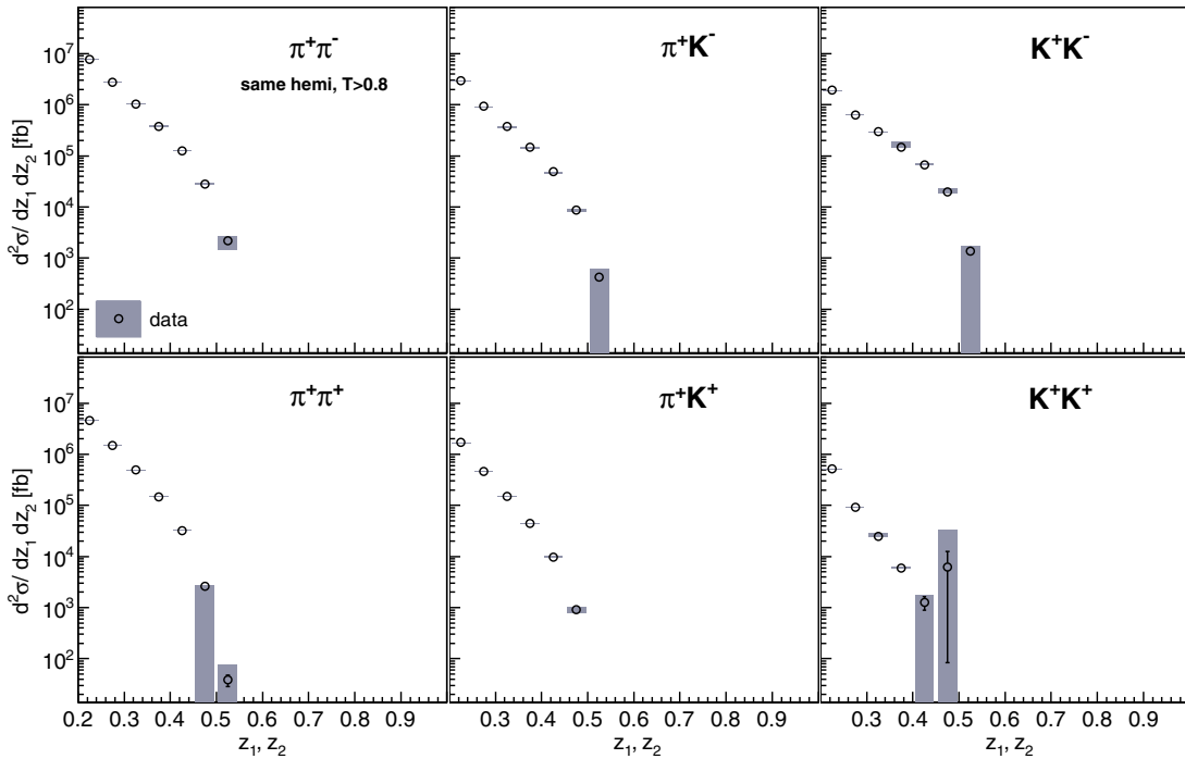
FIG. 16 (color online). Differential cross sections for the main hadron pairs within the same hemisphere (including thrust selection T > 0.8 ) as a function of (z_1, z_2) for diagonal bins only. The error boxes represent the systematic uncertainties.
