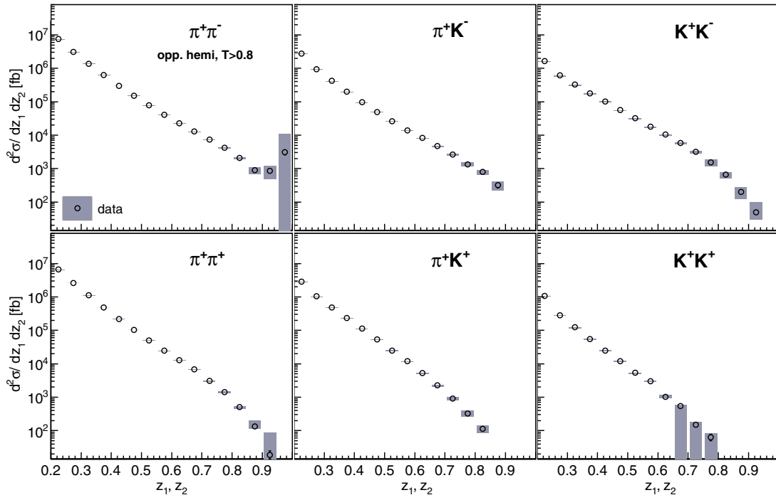
FIG. 15 (color online). Differential cross sections for the main hadron pairs within opposite hemispheres (including thrust selection T > 0.8 ) as a function of (z_1, z_2) for diagonal bins only. The error boxes represent the systematic uncertainties.
