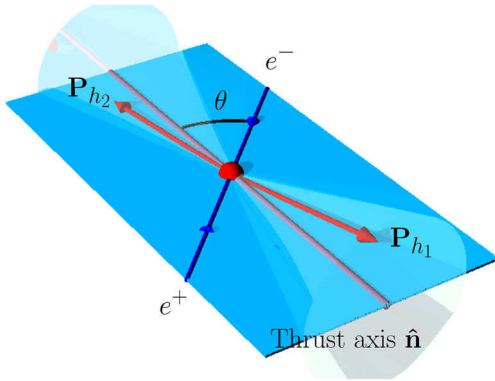
FIG. 1 (color online). Illustration of dihadron fragmentation where the final-state hadrons are depicted as red arrows, the incoming leptons as blue arrows, and the event plane—spanned by leptons and thrust axis—is depicted as a light blue plane. In this case, both hadrons are found in opposite hemispheres defined by the thrust axis, and generally out of the plane, as indicated by the cones.
