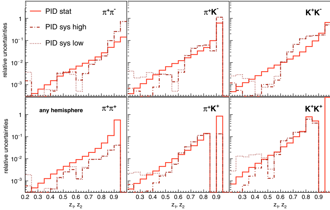
FIG. 4 (color online). Statistical (full lines), upper (dashed lines) and lower (red, dotted lines) systematic uncertainties relative to the PID-corrected dihadron yields in any topology as a function of ( z_1 = z_2 ); the diagonal bins of each two-dimensional matrix is shown for brevity. Empty bins are visible where the yields become zero, especially for high z bins.
