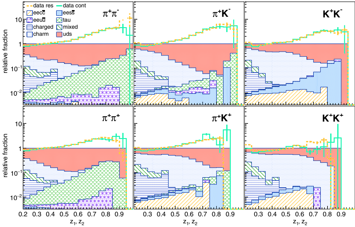
FIG. 6 (color online). Fraction of hadron pairs in any topology as a function of (z_1, z_2) originating from various subprocesses. The individual relative contributions are displayed from top to bottom for uds (red filled area), charm (blue, dotted area), mixed [ \Upsilon(4S) \rightarrow B^0 \bar{B}^0 , dark-green, hatched area] and charged [ \Upsilon(4S) \rightarrow B^+ B^- , violet, horizontally hatched area], \tau pair (light green, scaled area), eeu\bar{u} (purple, starred area), ees\bar{s} (light blue, dotted area) and eec\bar{c} (orange hatched area) events. Also, for comparison, the continuum (green, solid lines) and on-resonance (orange, dotted lines) data are shown. For brevity, only diagonal ( z_1 = z_2 ) entries in each two-dimensional matrix are shown.
