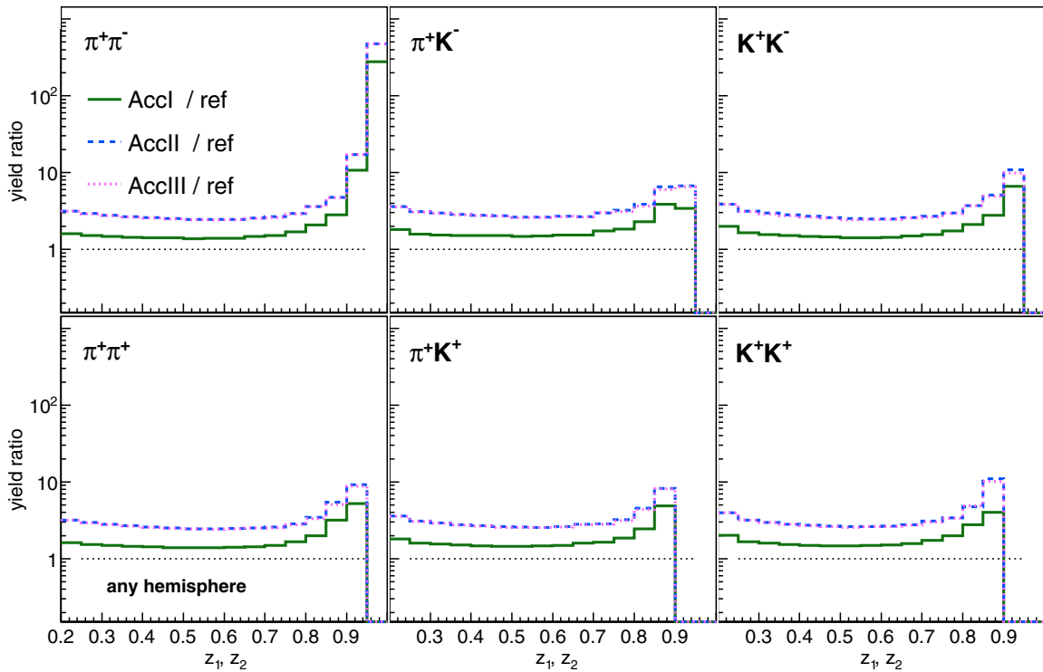
FIG. 7 (color online). Yield ratios after successively applying all acceptance and efficiency corrections (labeled AcclI to AcclIII as the three acceptance corrections discussed in the text) relative to the reference yields before (non- q\bar{q} removal) for various hadron combinations without hemisphere assignment. For brevity, only diagonal ( z_1 = z_2 ) entries in the two-dimensional matrices are shown.
