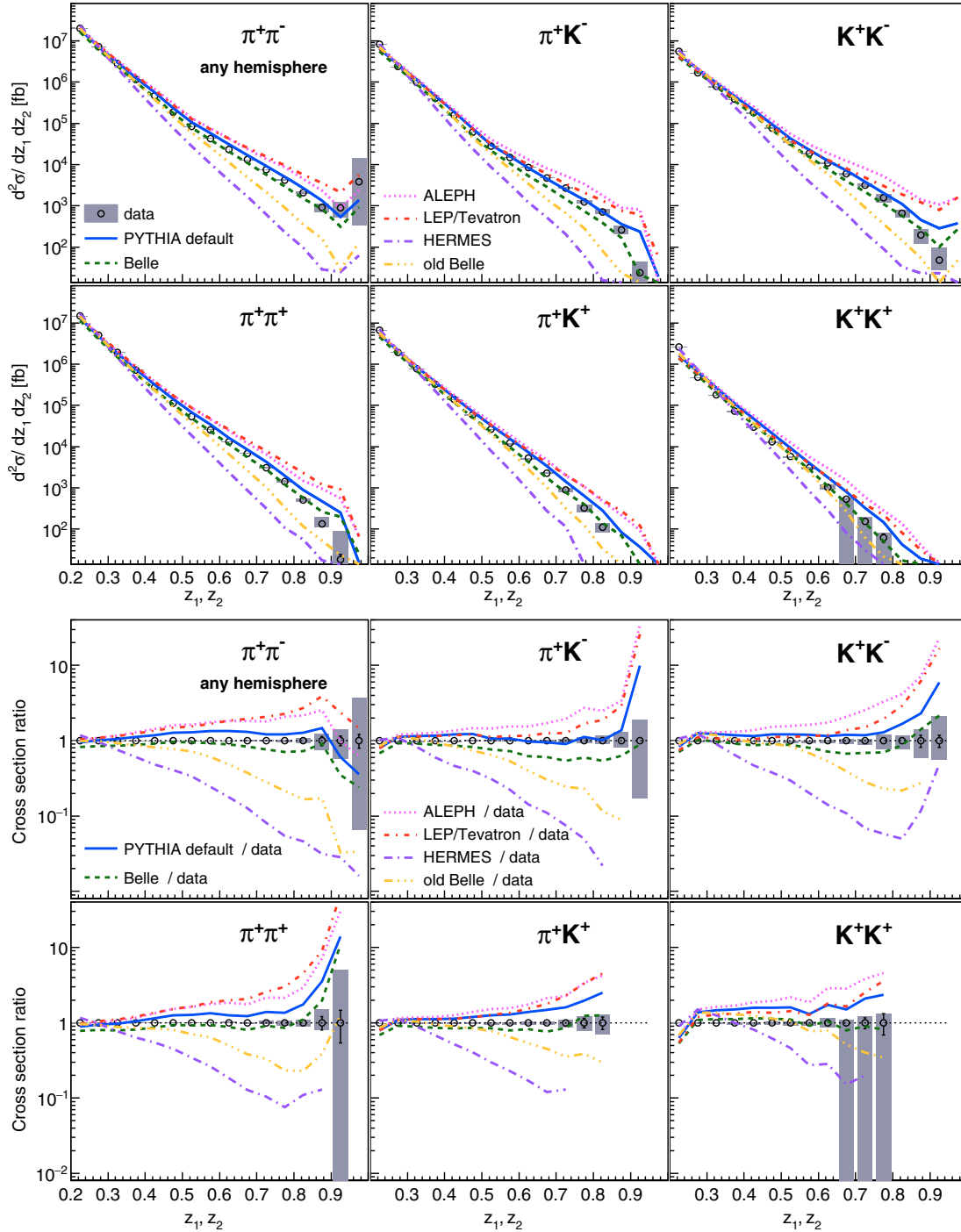
FIG. 18 (color online). Differential cross sections (top panels) and ratios to the data (bottom panels) for the main hadron pairs in the any topology as a function of (z_1, z_2) for diagonal bins only. Various PYTHIA tunes are also displayed as described in the text. For comparison, the relative statistical and systematic uncertainties are shown for the data as well.
