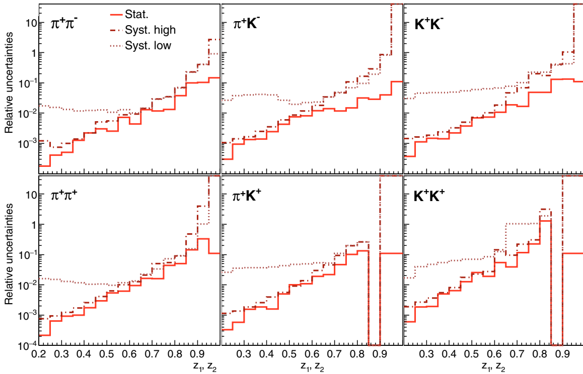
FIG. 11 (color online). Relative (asymmetric) systematic (lower uncertainties: dashed lines; upper uncertainties: dash-dotted lines) and statistical uncertainties (full lines) for the most relevant hadron pairs in the any topology as a function of (z_1, z_2) . For brevity, only the diagonal bins ( z_1 = z_2 ) are shown.
