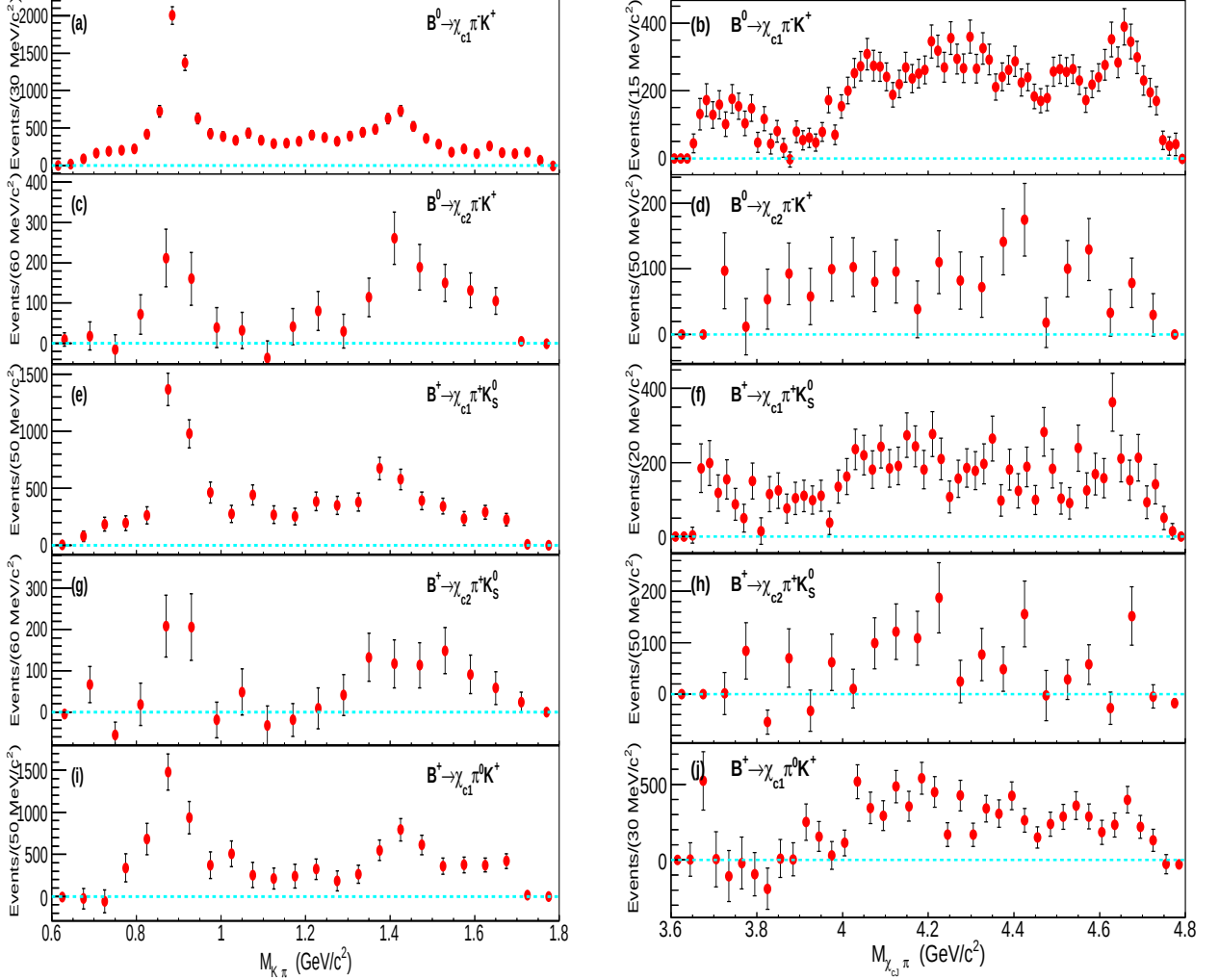
FIG. 4: (color online) Background subtracted efficiency corrected s\mathcal{P}lot M_{K\pi} and M_{\chi\pi} distributions for the (a and b) B^0 \rightarrow \chi_{c1} \pi^- K^+ , (c and d) B^0 \rightarrow \chi_{c2} \pi^- K^+ , (e and f) B^+ \rightarrow \chi_{c1} \pi^+ K_S^0 , (g and h) B^+ \rightarrow \chi_{c2} \pi^+ K_S^0 and (i and j) B^+ \rightarrow \chi_{c1} \pi^0 K^+ decay modes.
