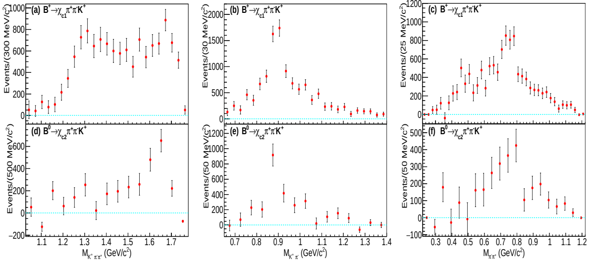
FIG. 7: (color online) Background subtracted efficiency corrected s\mathcal{P}lot (a and d) M_{K^+\pi^+\pi^-} , (b and e) M_{K^+\pi^-} and (c and f) M_{\pi^+\pi^-} distributions for B^+ \rightarrow \chi_{c1}\pi^+\pi^-K^+ decay (upper) and B^+ \rightarrow \chi_{c2}\pi^+\pi^-K^+ decay (lower), respectively.
