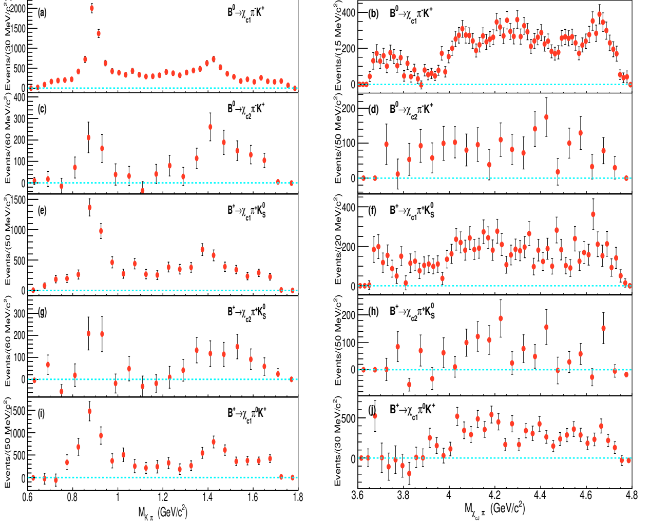
FIG. 4: (color online) Background subtracted efficiency corrected s\mathcal{P}lot M_{K\pi} and M_{\chi_{cJ}\pi} distributions for the (a and b) B^0 \rightarrow \chi_{c1}\pi^- K^+ , (c and d) B^0 \rightarrow \chi_{c2}\pi^- K^+ , (e and f) B^+ \rightarrow \chi_{c1}\pi^+ K_S^0 , (g and h) B^+ \rightarrow \chi_{c2}\pi^+ K_S^0 and (i and j) B^+ \rightarrow \chi_{c1}\pi^0 K^+ decay modes.
