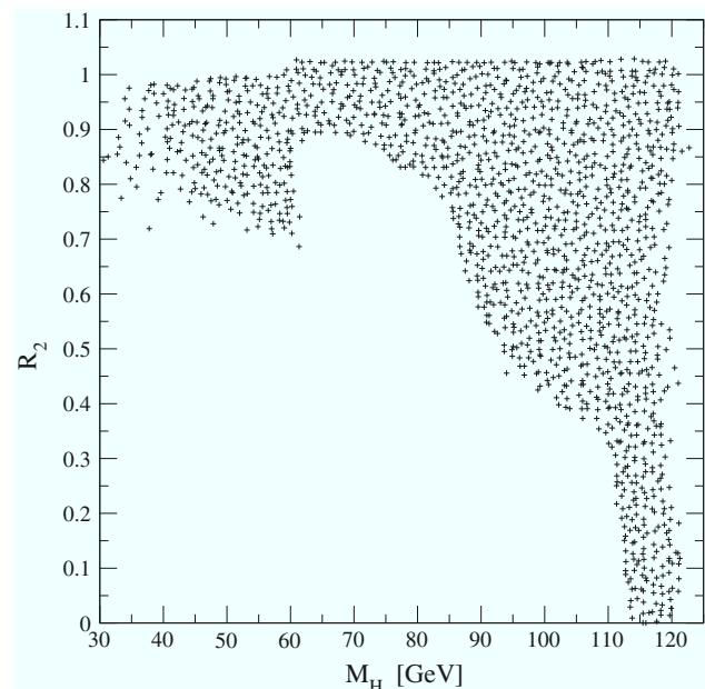
Fig. 88 The reduced signal cross section R_2^{bb} as function of M_{H_1} in the semiconstrained NMSSM (from [482]).
