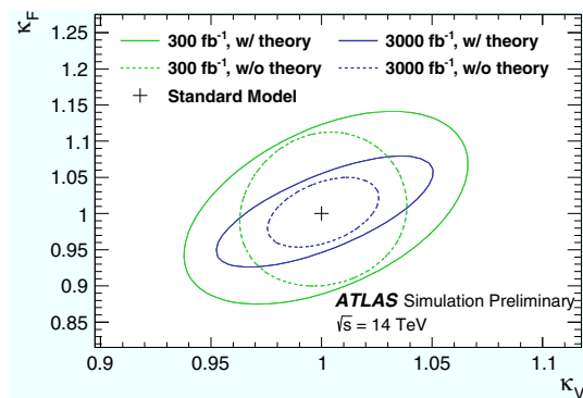
Fig. 32 Expected ATLAS 68 and 95 % CL likelihood contours for \kappa_V and \kappa_F in a minimal coupling fit for an integrated luminosity of 300 fb -1 and 3000 fb -1 [136]
