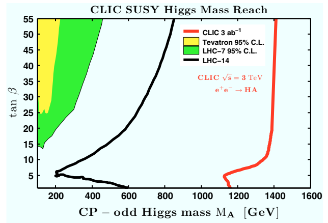
Fig. 58 Search reach in the m_A - \tan\beta plane for LHC and CLIC. The left-most coloured regions are current limits from the Tevatron with \sim 7.5 \text{ fb}^{-1} of data at \sqrt{s} = 1.96 TeV and from \sim 1 \text{ fb}^{-1} of LHC data at \sqrt{s} = 7 TeV. The black line is projection of search reach at LHC with \sqrt{s} = 14 TeV and 300 \text{ fb}^{-1} of luminosity [211]. The right-most red line is search reach of CLIC in the HA mode with \sqrt{s} = 3 TeV. This search capacity extends well beyond the LHC [9, 10]
