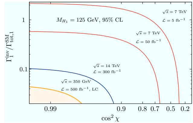
Fig. 85 95% confidence level contours for a measurement of \Gamma_1^{hid}/\Gamma_{tot,1}^{SM} at the LHC and a 350 GeV LC. We use SFITTER [459] for the LHC results and we adopt the linear collider uncertainties of reference [458]
