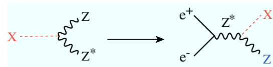
Fig. 38 X \rightarrow ZZ^* decay and e^+e^- \rightarrow ZX process
