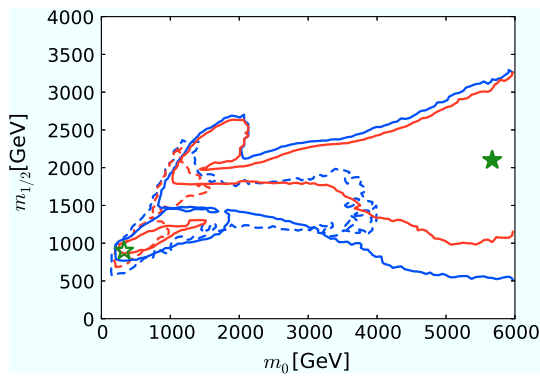
Fig. 155 The (m_0, m_{1/2}) planes in the CMSSM including the ATLAS 20/fb jets + \cancel{E}_T , \text{BR}(B_{s,d} \rightarrow \mu^+ \mu^-) , m_h , \Omega_\chi h^2 , LUX, and other constraints. The most recent results are indicated by solid lines and filled stars, and previous fit based on \sim 5/\text{fb} of LHC data is indicated by dashed lines and open stars. The blue lines denote 68% CL contours, and the red lines denote 95% CL contours
