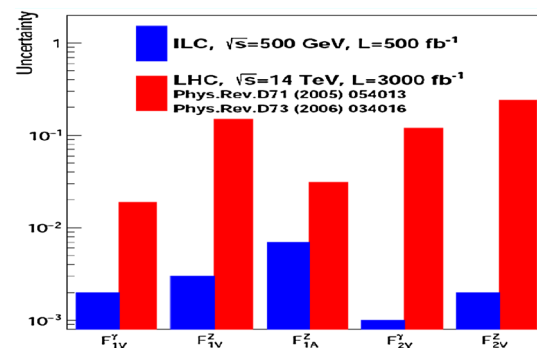
Fig. 3 Statistical precision on CP -conserving form factors expected at the LHC [42] and at the ILC [41]. The LHC results assume an integrated luminosity of \mathcal{L} = 3000 \text{ fb}^{-1} . The results for the ILC are based on an integrated luminosity of \mathcal{L} = 500 \text{ fb}^{-1} at \sqrt{s} = 500 \text{ GeV} and a beam polarisation of P_{e^-} = \pm 80\% , P_{e^+} = \mp 30\% [41]
