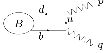
Figure 10: Correlation function with B-meson DA's
